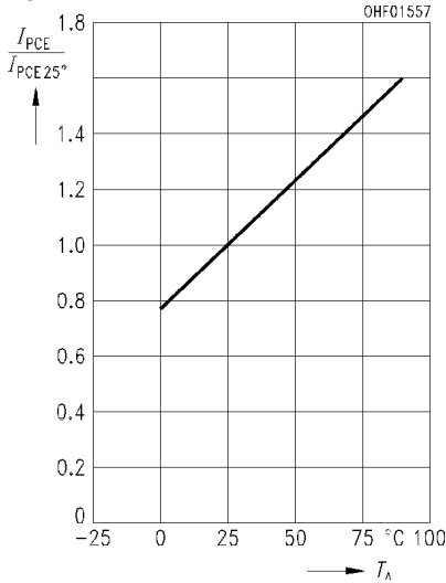
Photocurrent I_{PCE}/I_{PCE25^\circ} = f(T_A) , V_{CE} = 5 \text{ V}
