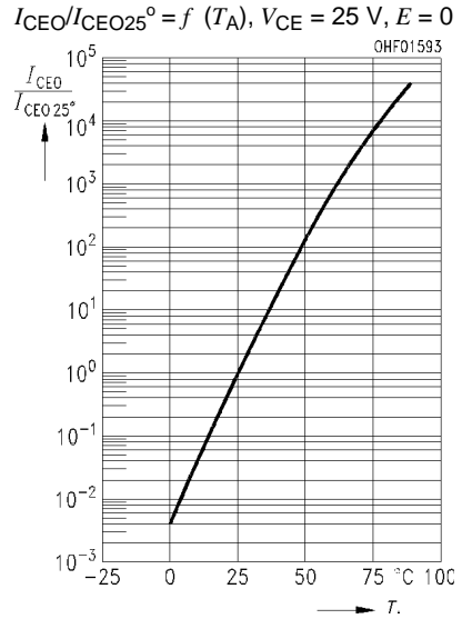
Dark current
