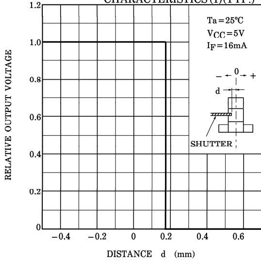
TLP1006A DETECTING POSITION CHARACTERISTICS (1)(TYP.)
