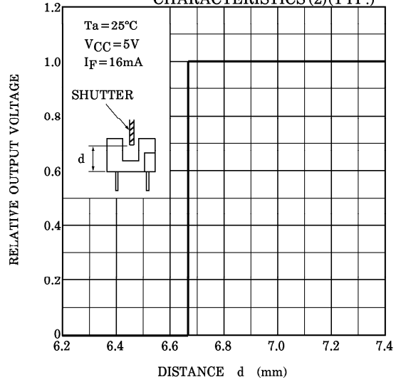
TLP1006A DETECTING POSITION CHARACTERISTICS (2)(TYP.)
