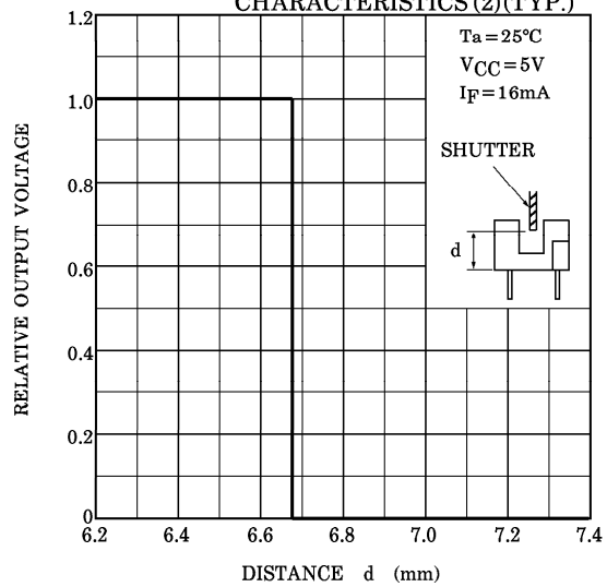
TLP1007A DETECTING POSITION CHARACTERISTICS (2)(TYP.)
