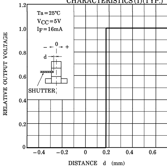
TLP1007A DETECTING POSITION CHARACTERISTICS (1)(TYP.)
