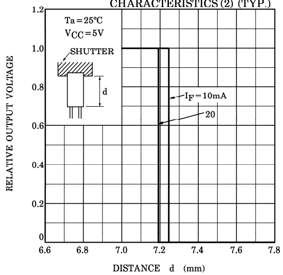
TLP1003A DETECTING POSITION CHARACTERISTICS (2) (TYP.)
