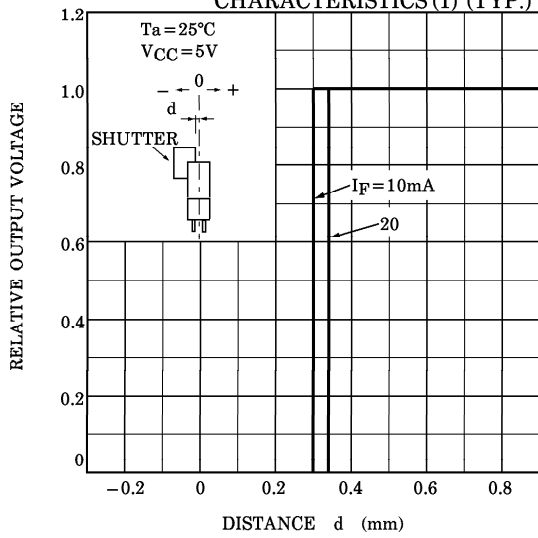
TLP1003A DETECTING POSITION CHARACTERISTICS (1) (TYP.)
