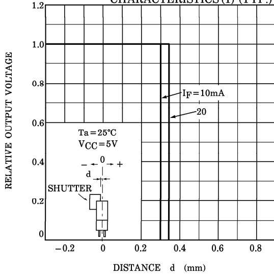
TLP1002A DETECTING POSITION CHARACTERISTICS (1) (TYP.)
