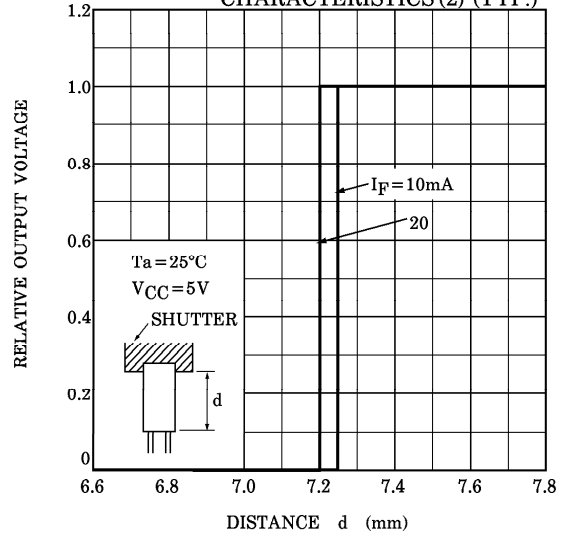
TLP1002A DETECTING POSITION CHARACTERISTICS (2) (TYP.)
