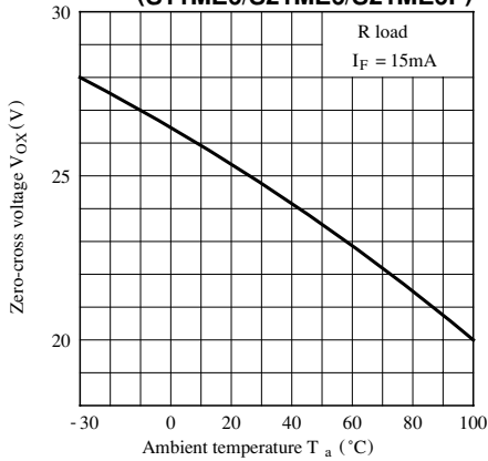
Fig11. Zero-cross Voltage vs. Ambient Temperature (S11ME6/S21ME6/S21ME6F)
