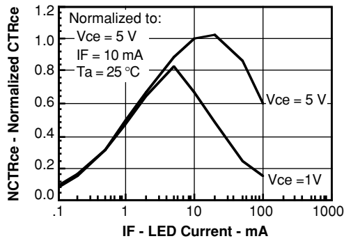
Figure 2. Normalized Non-saturated and Saturated CTR Rce versus LED Current
