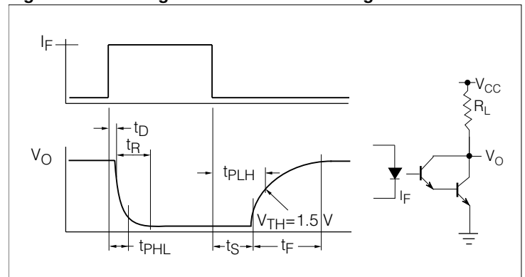
Figure 8. Switching Waveform and Switching Schematic
