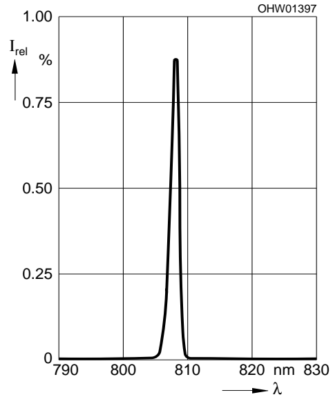
Optical Spectrum, Relative Intensity I_{rel} vs. Wavelength \lambda ( T_A = 25\text{ }^\circ\text{C} , P_{opt} = 1.5\text{ W} ) SPL 2F81-2S-105
