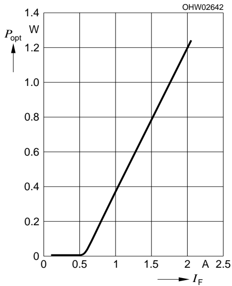
Optical Output Power P_{opt} vs. Forward Current I_F ( T_A = 25\text{ }^\circ\text{C} ) SPL 2F81-2S-105
