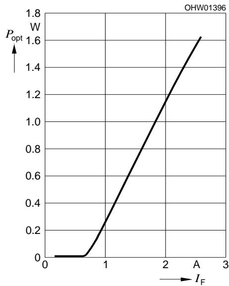
Optical Output Power P_{opt} vs. Forward Current I_F ( T_A = 25\text{ }^\circ\text{C} ) SPL 2F81-2S
