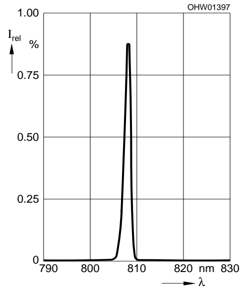
Optical Spectrum, Relative Intensity I_{rel} vs. Wavelength \lambda ( T_A = 25\text{ }^\circ\text{C} , P_{opt} = 1.5\text{ W} ) SPL 2F81-2S
