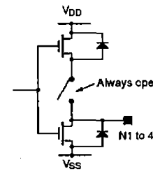
Figure 12. Port N open-drain outputs
