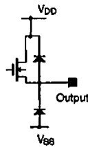
Figure 10. p-channel output
