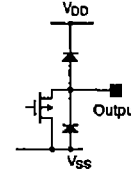
Figure 11. n-channel output
