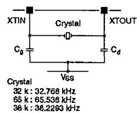
Figure 8. Crystal oscillator
