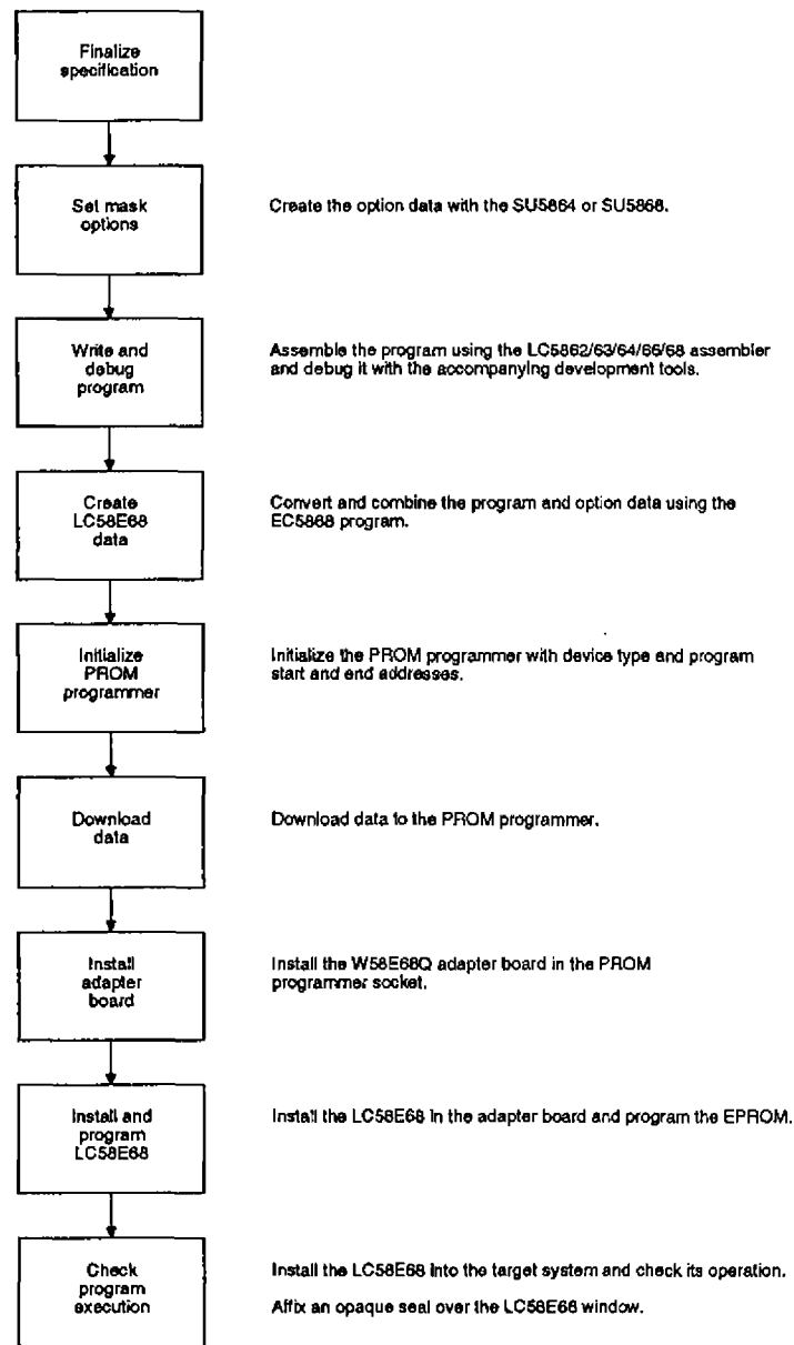
Figure 13. Development flowchart
