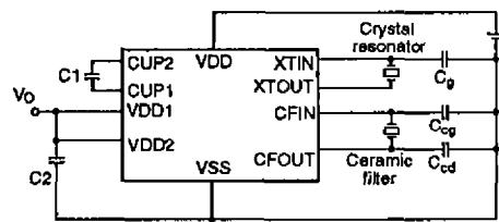
Figure 2. Output voltage measurement 1
