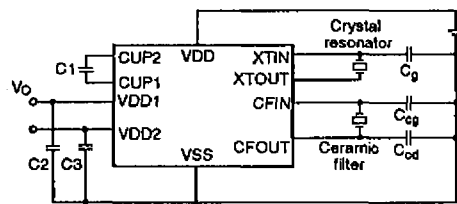
Figure 3. Output voltage measurement 2
