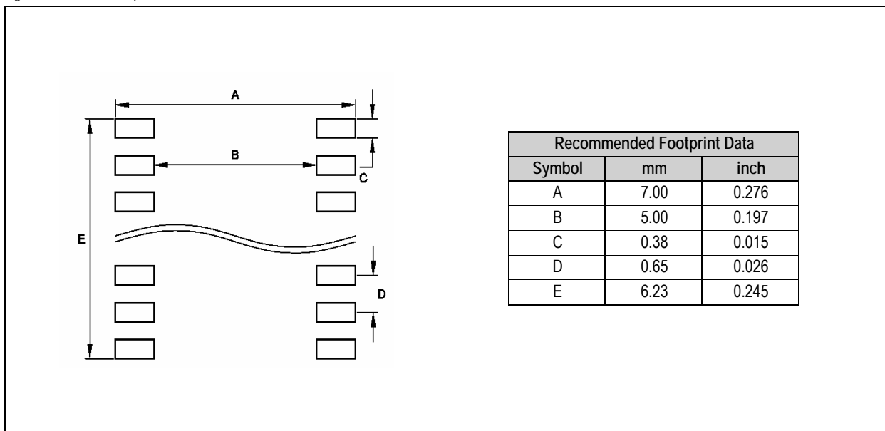
Figure 18. PCB Footprint
