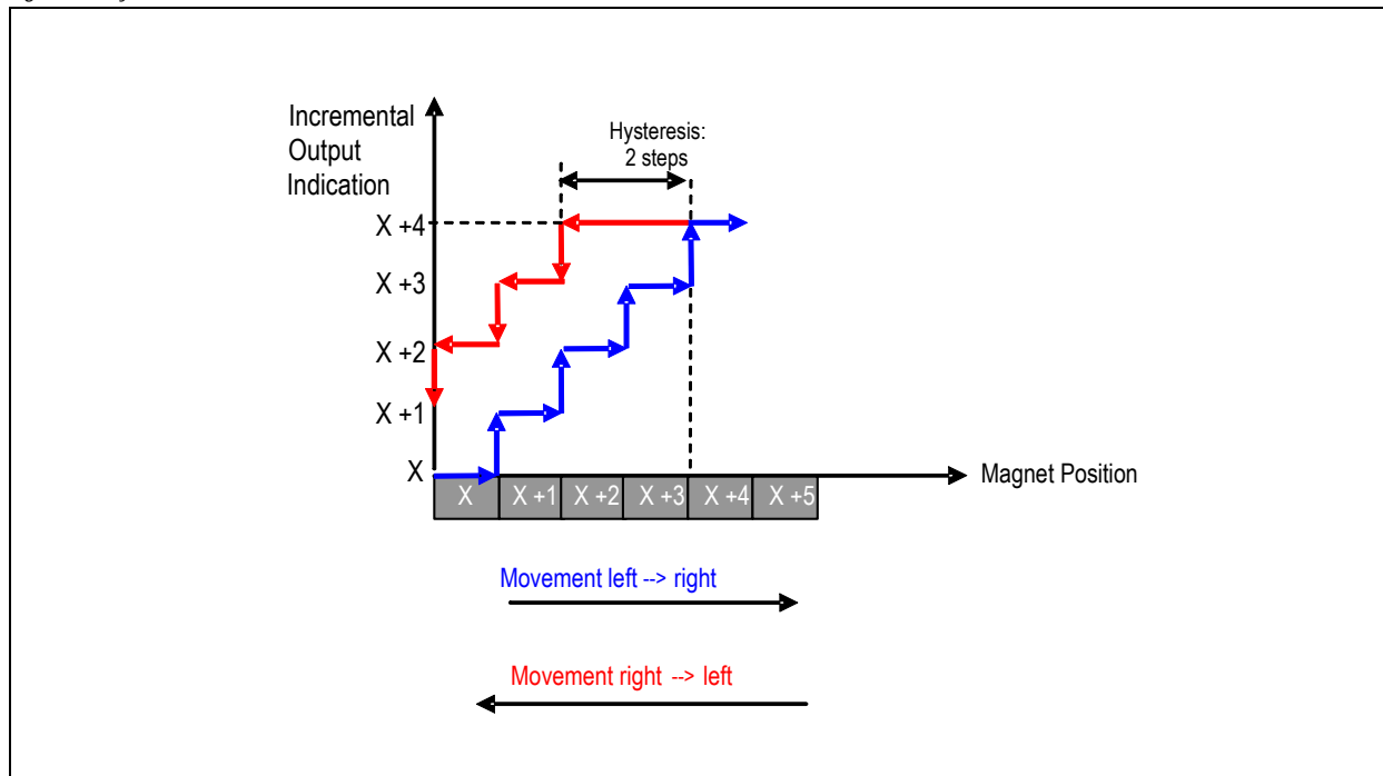
Figure 5. Hysteresis Illustration
