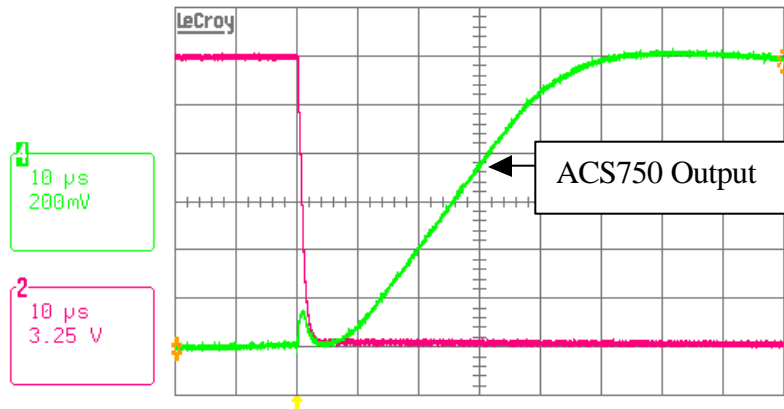
Step Resonance, I_{PRIMARY} = 50A
