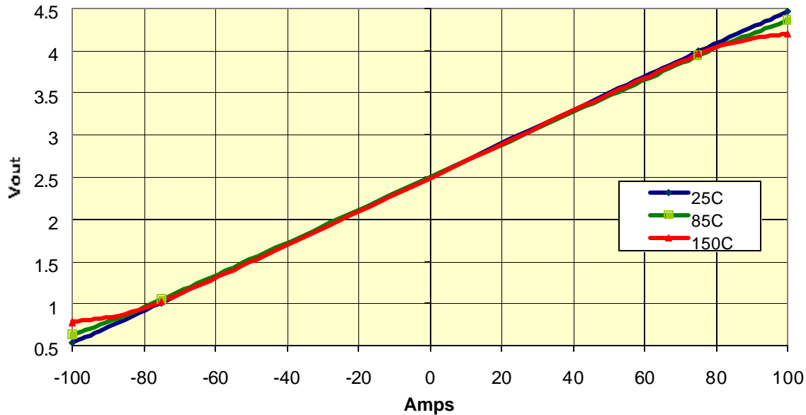
Figure 4: Primary current versus typical sensitivity across temperature
