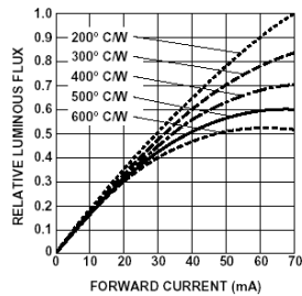
Figure 4. HPWT-xx00 Relative Luminous Flux vs. Forward Current.
