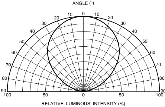
Fig.1 Directional pattern
