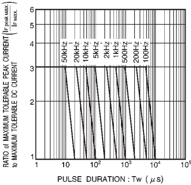
Fig. 19 Maximum tolerable peak current vs. pulse duration
