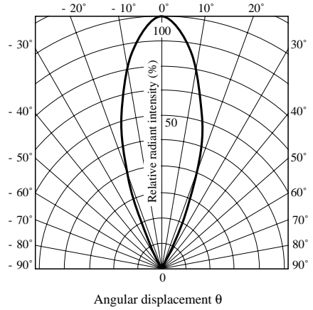
Fig. 8 Radiation Diagram
