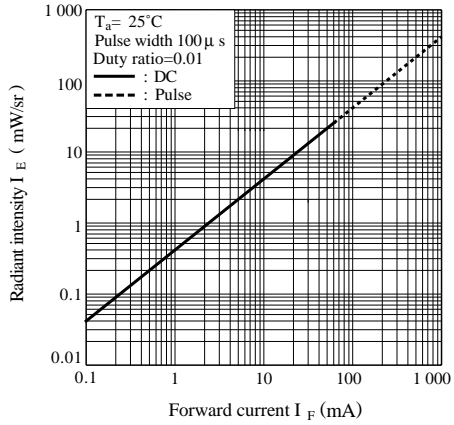
Fig. 7 Radiant Intensity vs. Forward Current
