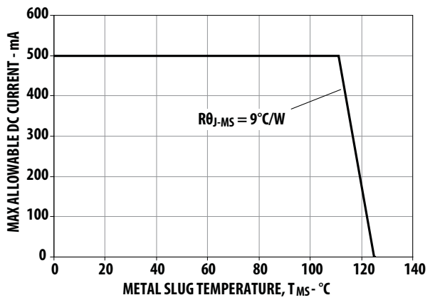
Figure 11. Maximum Forward Current vs. Ambient Slug Temperature. Derated based on T JMAX = 125°C, R θJ-MS = 9°C/W
