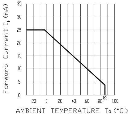
Forward Current Derating Curve T_a=25^\circ
