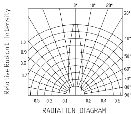
Radiation Diagram T a =25°C
