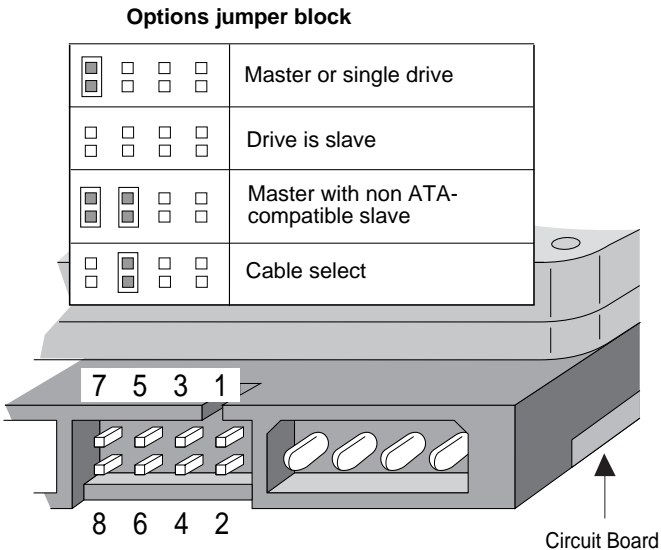
Figure 2. Master/slave jumper settings
