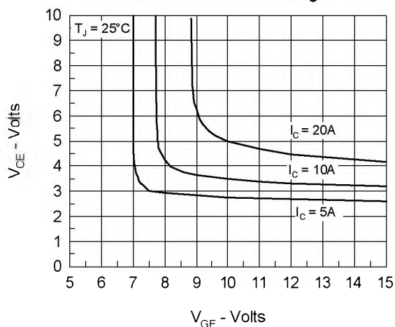
Fig. 3 Collector-Emitter Voltage vs. Gate-Emittor Voltage
