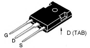
TO-247 AD
