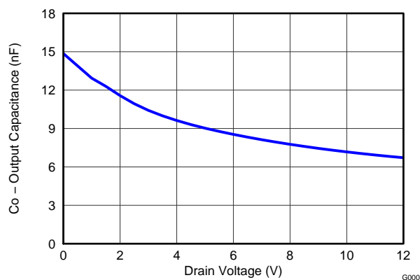
Figure 6. Output Capacitance
