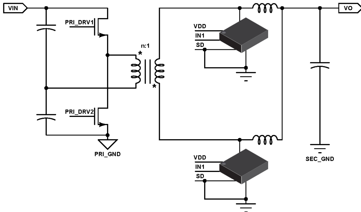
Figure 1. Application Diagram
