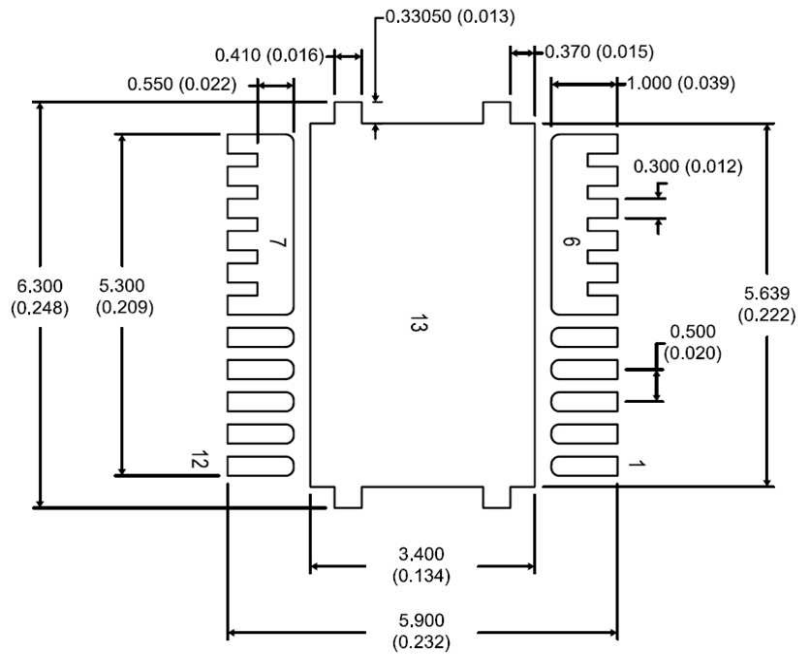
RECOMMENDED PCB LAND PATTERN
