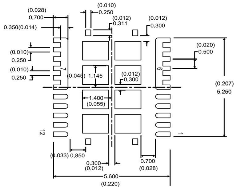
STENCIL OPENING RECOMMENDATION
