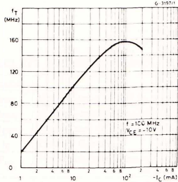
Transition Frequency.
