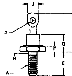
DO-203AA (DO-4)
