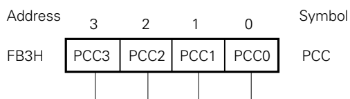
Fig. 4-12 Format of the Processor Clock Control Register
