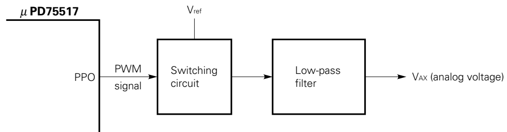
Fig. 4-33 Sample Configuration of D/A Conversion Using \mu PD75517
