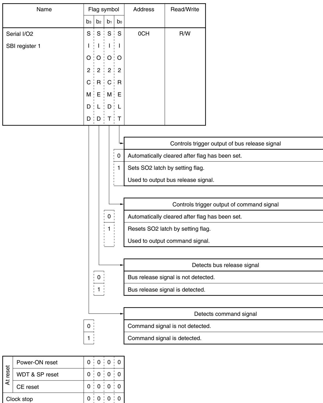
Figure 16-6. Configuration of Serial I/O2SBI Register
