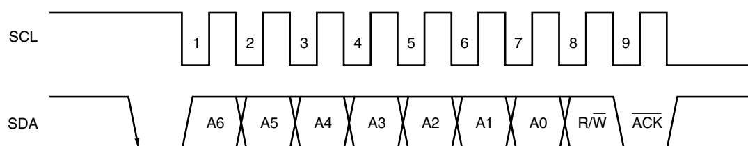
Figure 16-44. Acknowledge Signal
