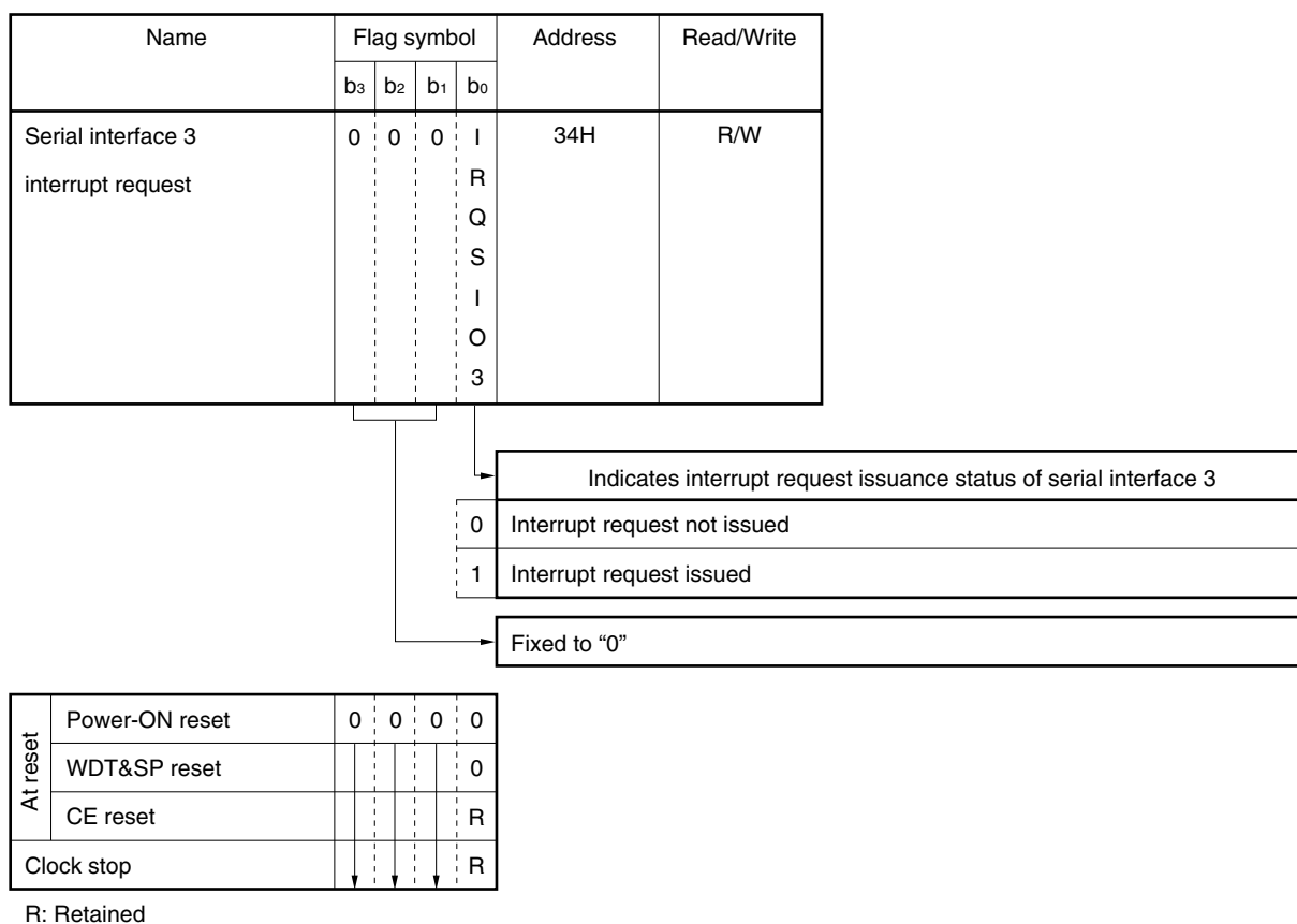
Figure 12-2. Configuration of Serial Interface 3 Interrupt Request Register
