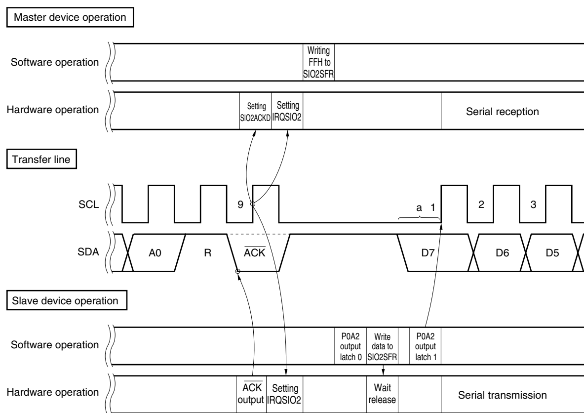
Figure 16-51. Slave Wait Release (Transmission)
