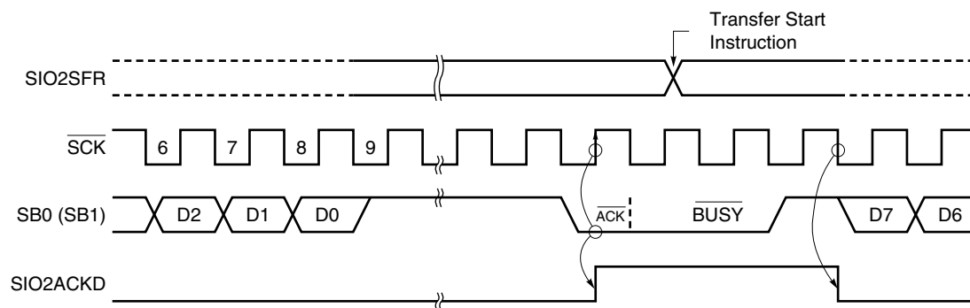
Figure 16-30. SIO2BSYE Operation
