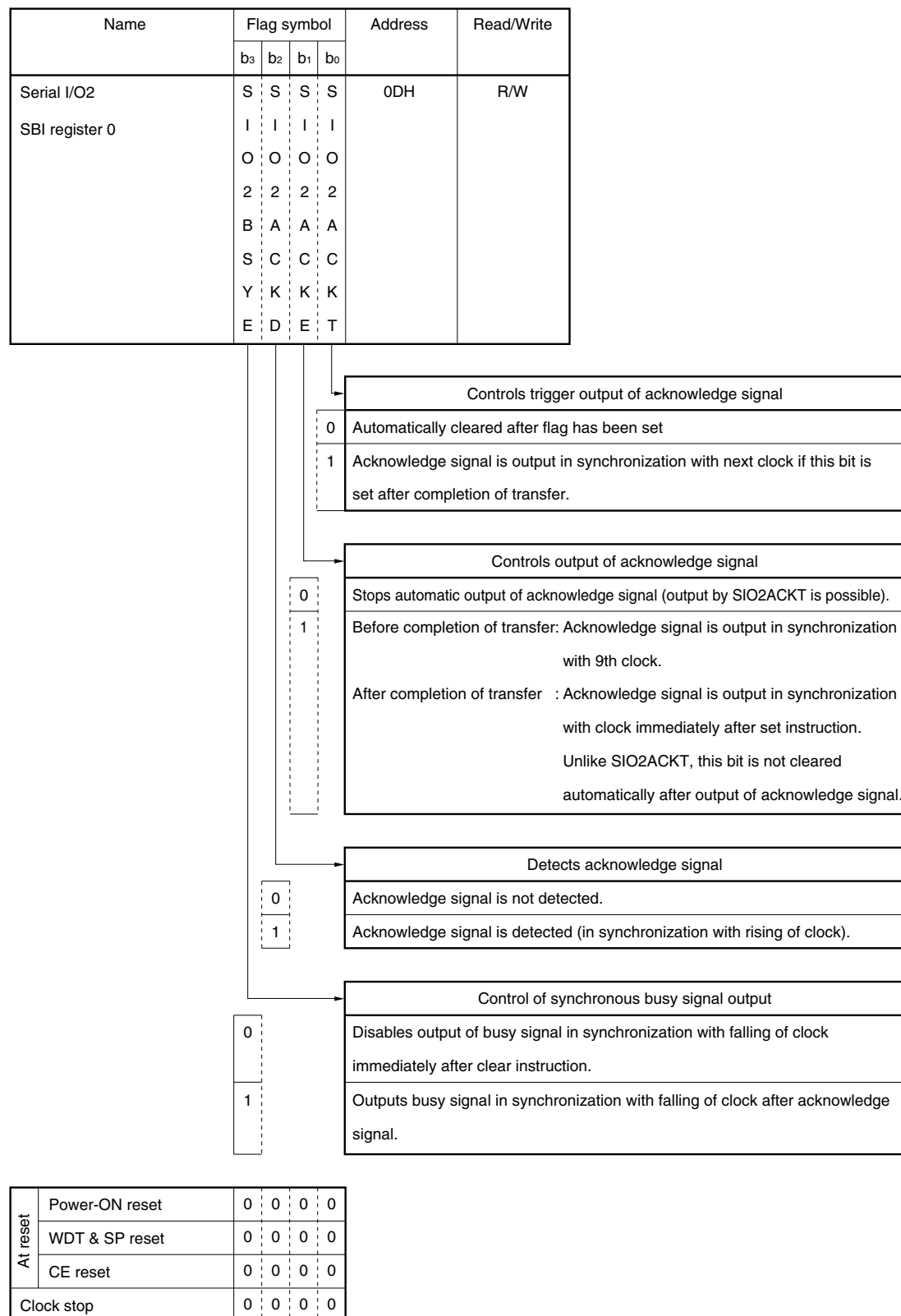
Figure 16-5. Configuration of Serial I/O2SBI Register 0
