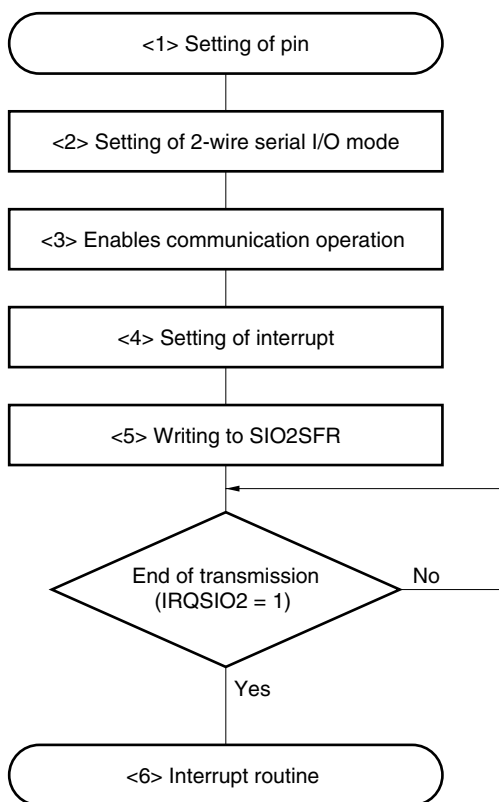
Figure 16-38. Example Flowchart in 2-Wire Serial I/O Transmission Mode
