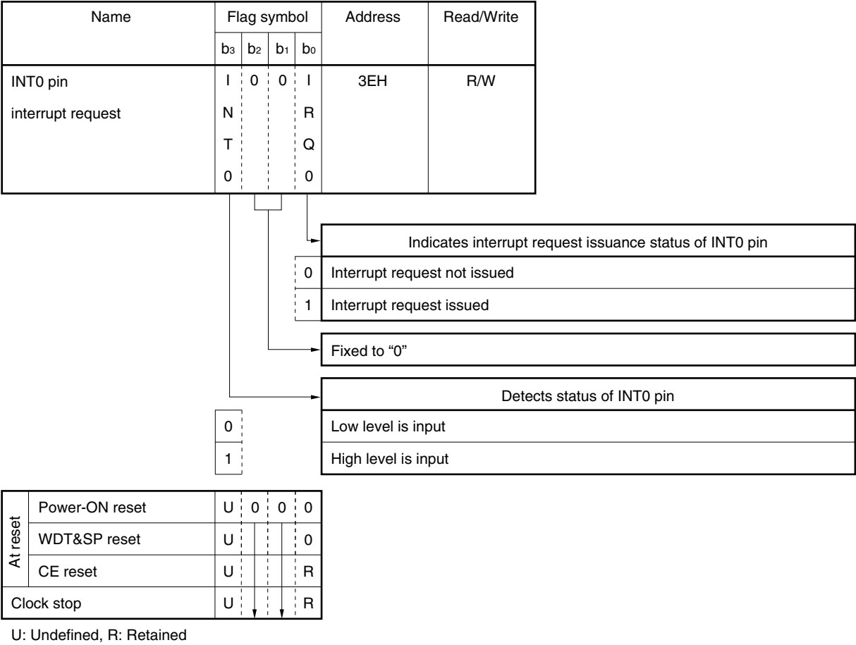
Figure 12-12. Configuration of INT0 Pin Interrupt Request Register
