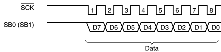
Figure 16-22. Data
