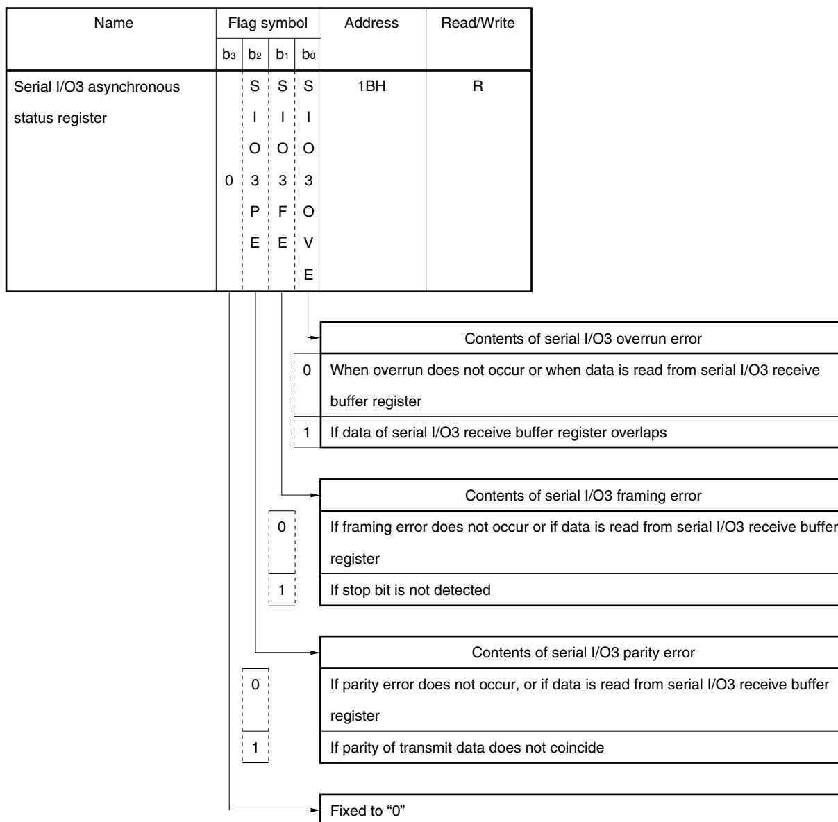
Figure 16-59. Configuration of Serial I/O3 Asynchronous Status Register
