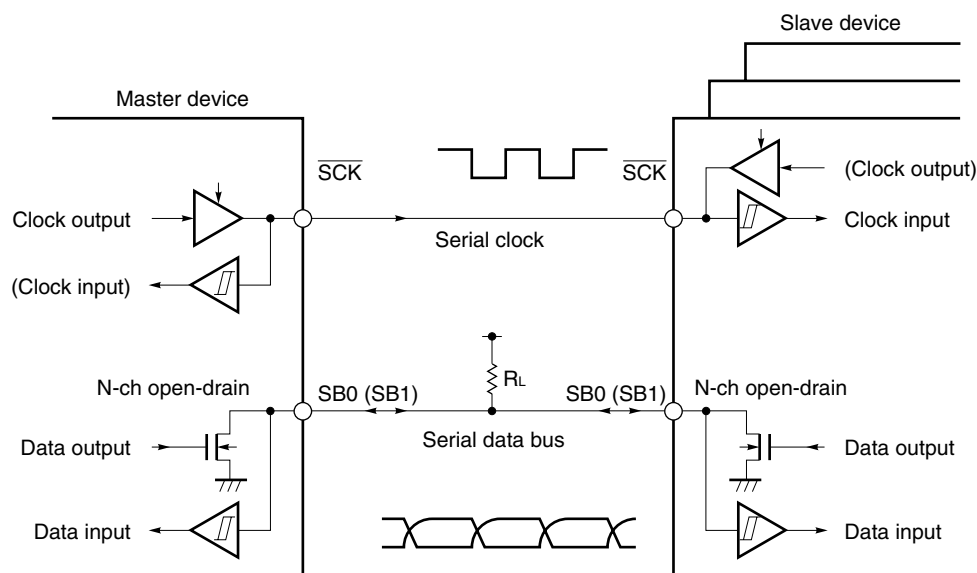
Figure 16-31. Pin Configuration
