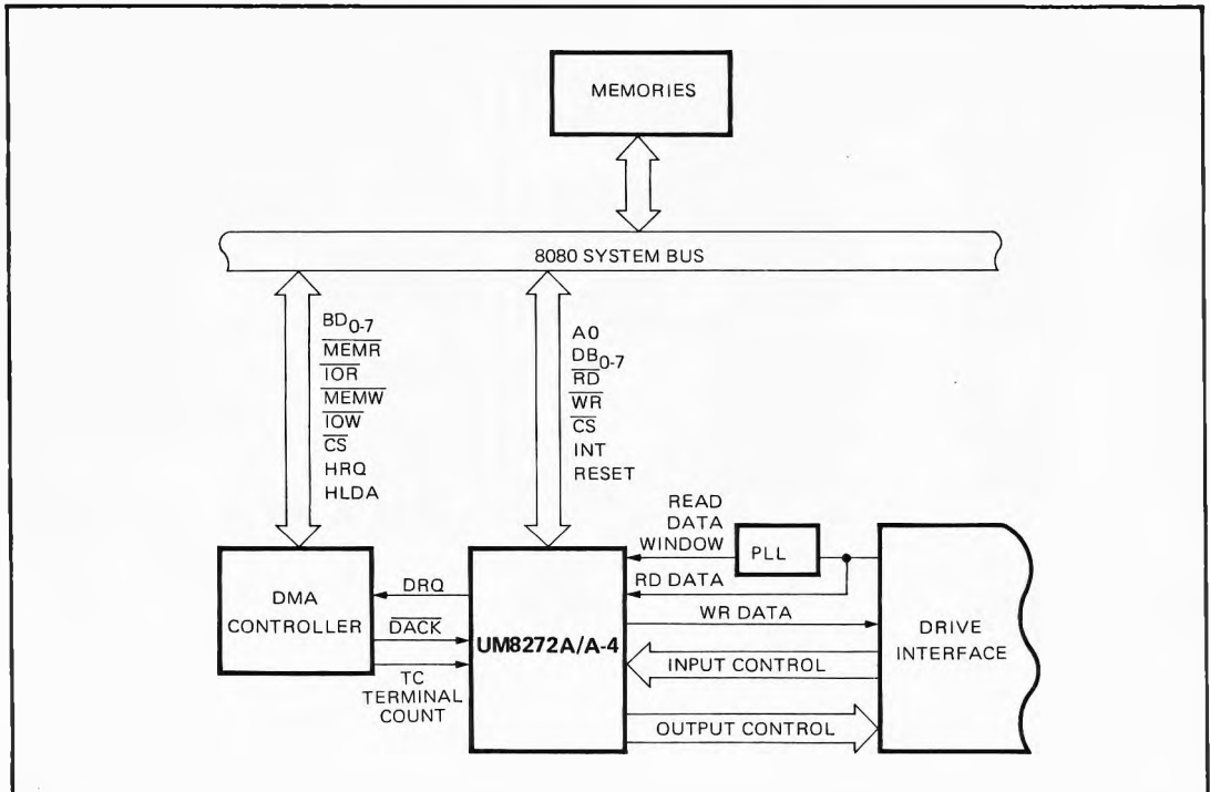
Figure 1. System Configuration
