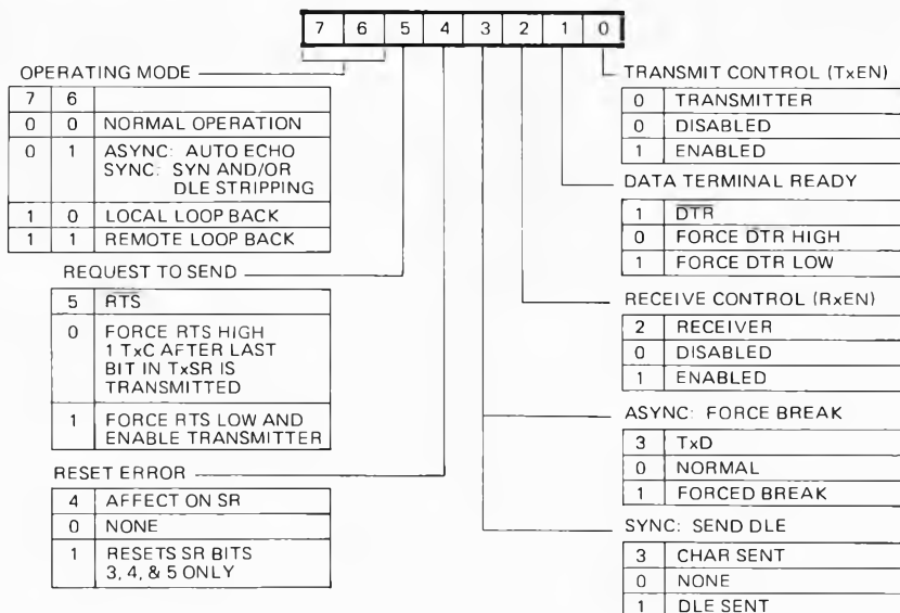
Figure 10. Command Register
