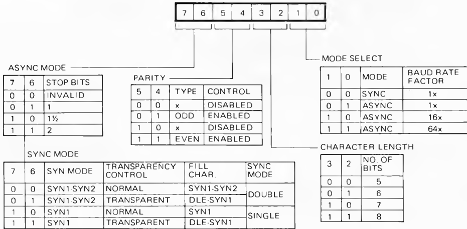
Figure 8. Mode Register 1
