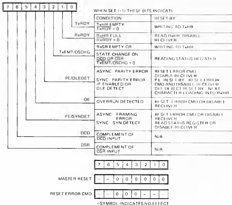
Figure 11. Status Register
