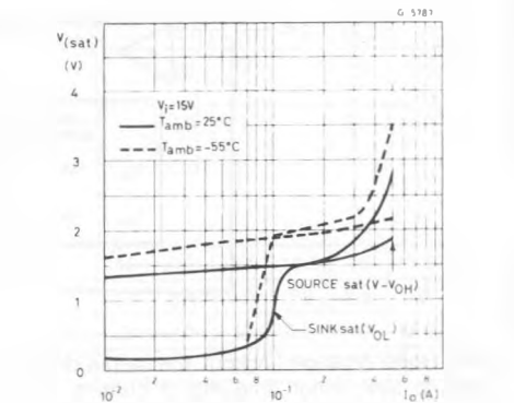
Figure 7 : Output Saturation Characteristics.
