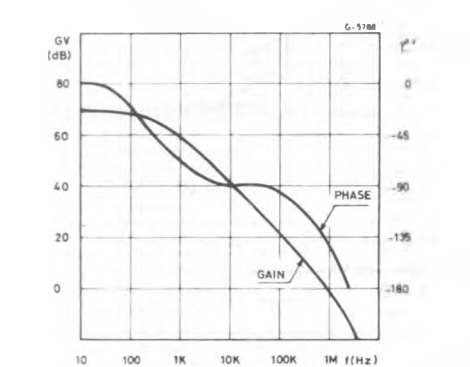
Figure 8 : Error Amplifier Open-loop Frequency Response.
