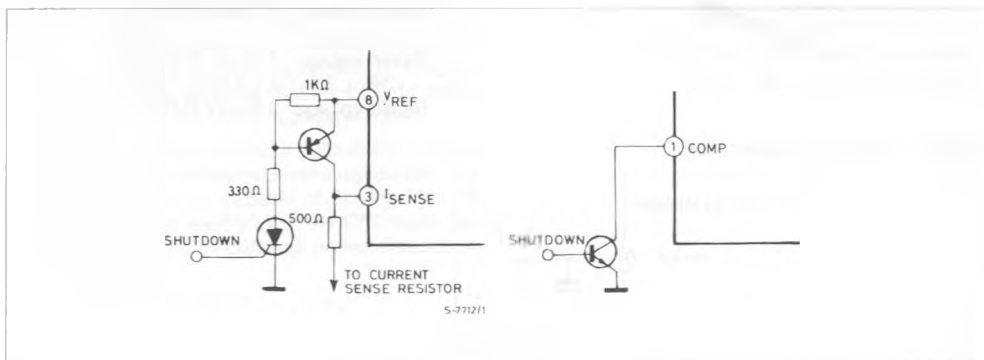
Figure 10 : Shutdown Techniques.
