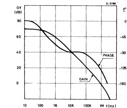
Figure 8 : Error Amplifier Open-loop Frequency Response.
