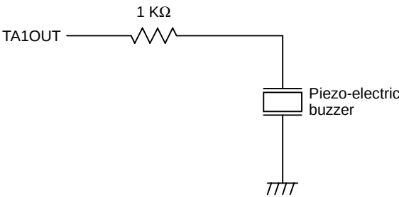
Figure 2.3.10 Piezo-electric buzzer
