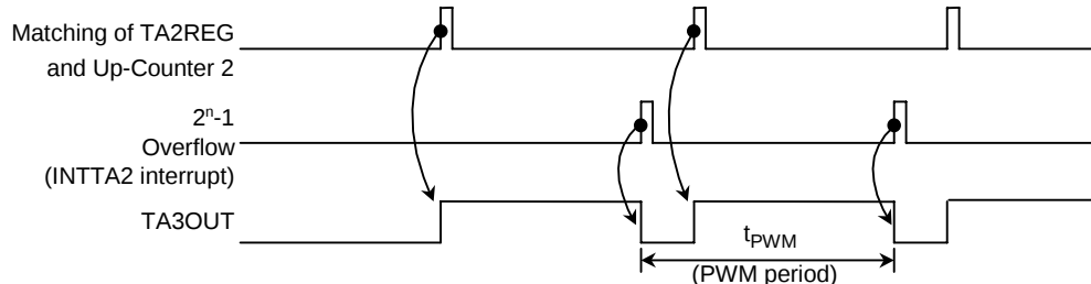
Figure 3.2.8 PWM timing waveform
