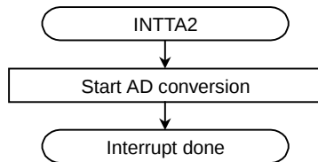
Figure 3.6.14 INTTA2 interrupt processing
