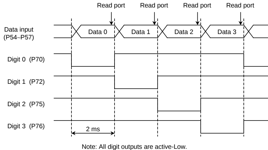
Figure 3.3.12 Timing chart for reading in data and changing the digits
