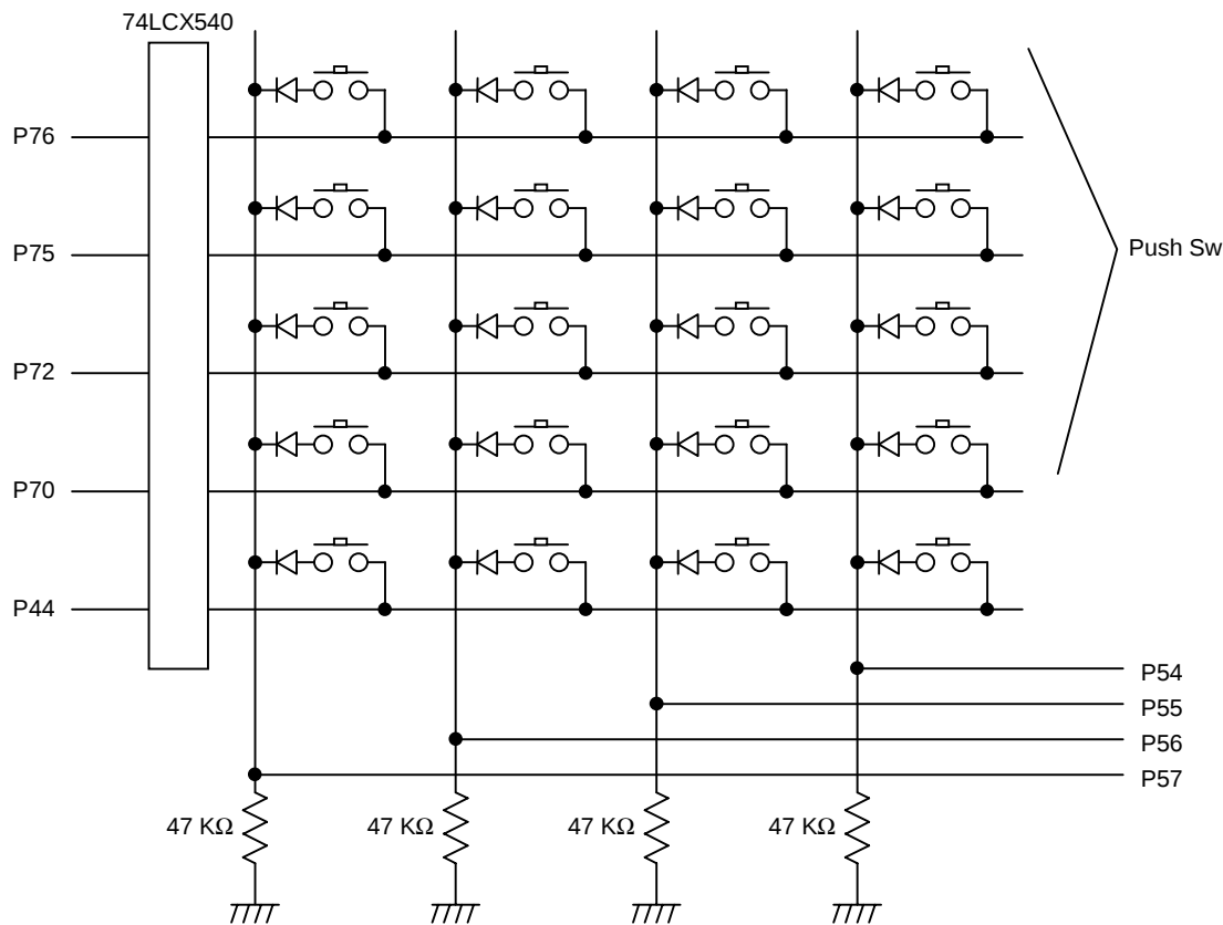
Figure 2.3.9 Diode matrix key switch
