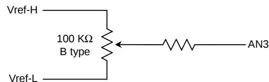
Figure 2.3.4 Volume control
