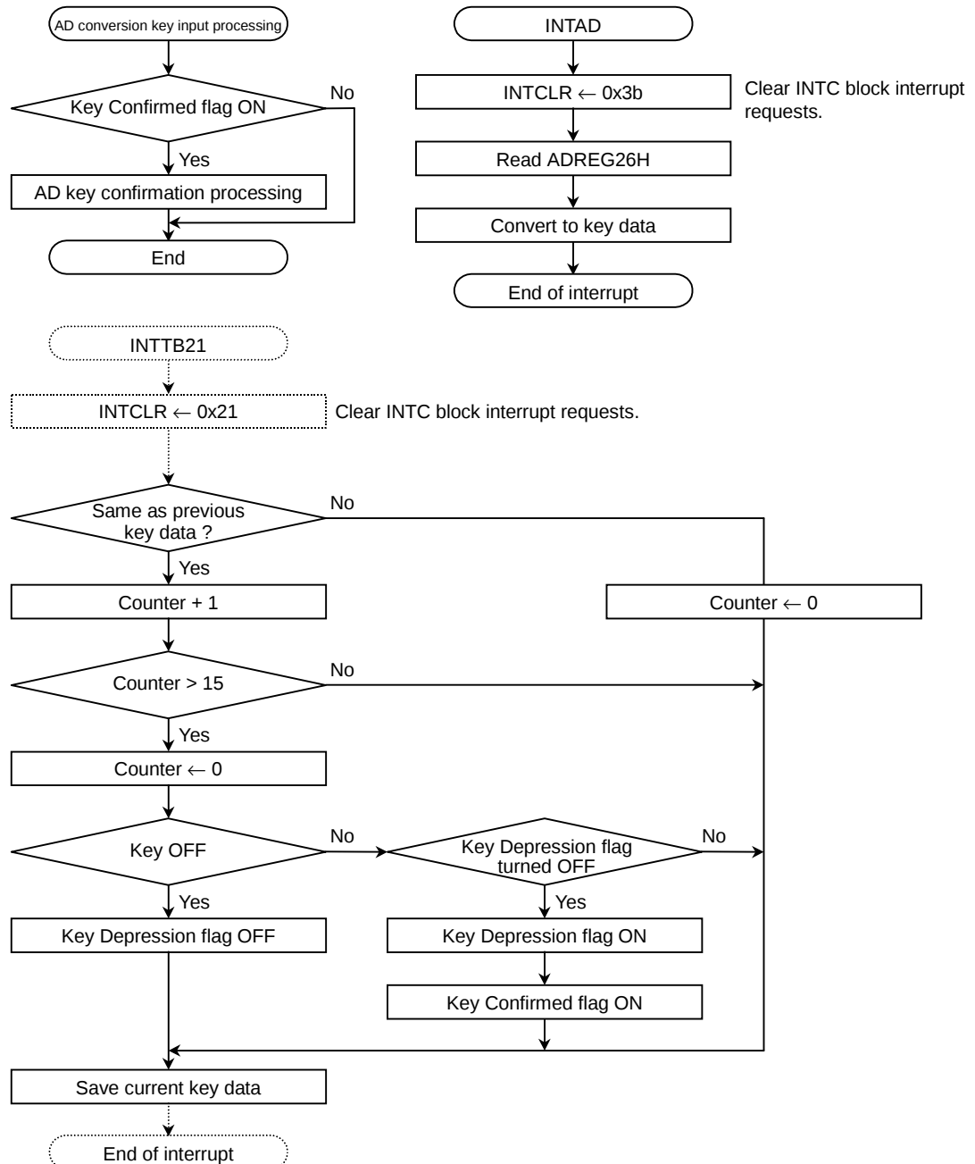
Figure 3.4.7 Operation flow for control of AD conversion key input
