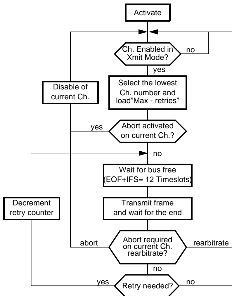
Figure 26. Transmit Function
