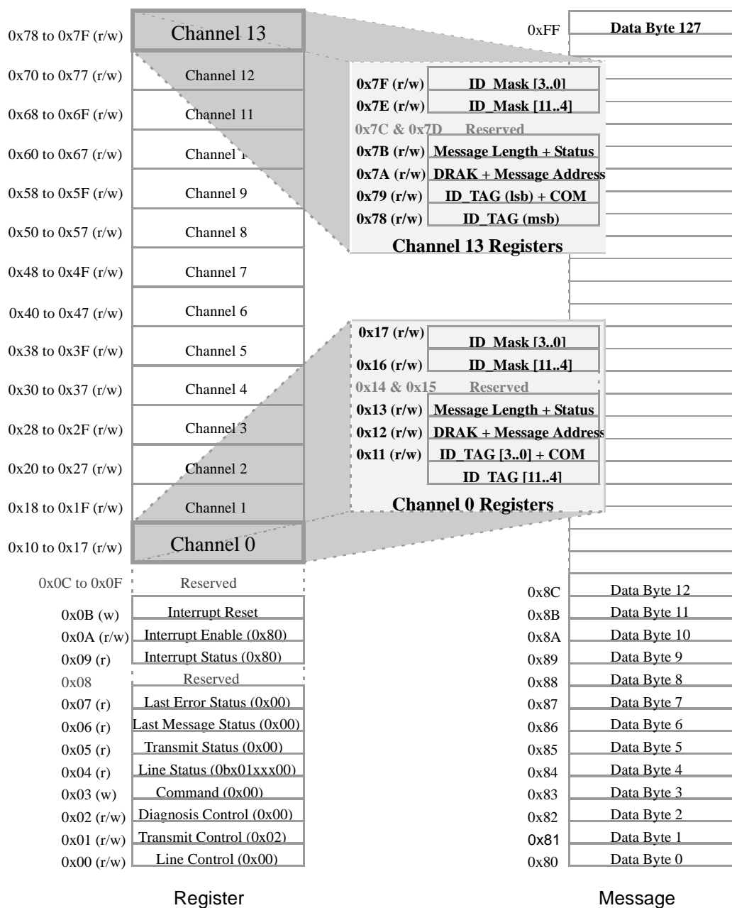
Figure 18. Memory Map
