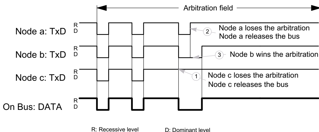
Figure 6. CSMA/CD Arbitration
