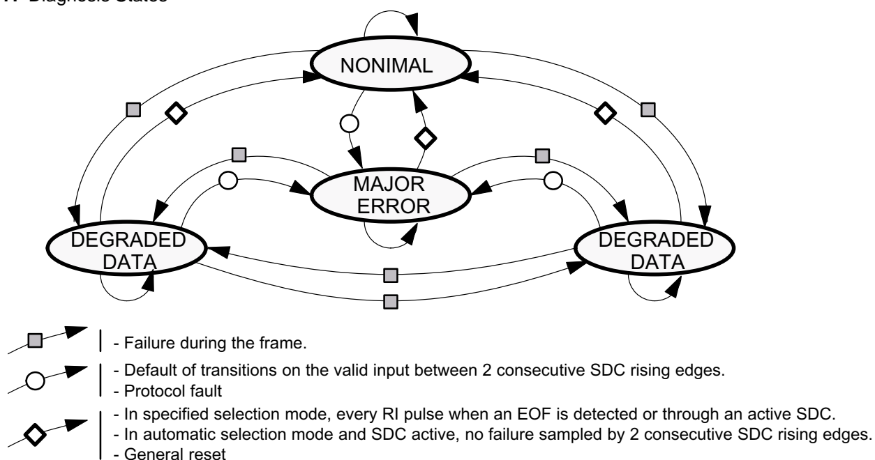
Figure 17. Diagnosis States
