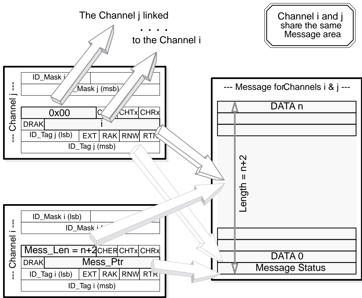
Figure 32. Linkage Mechanism
