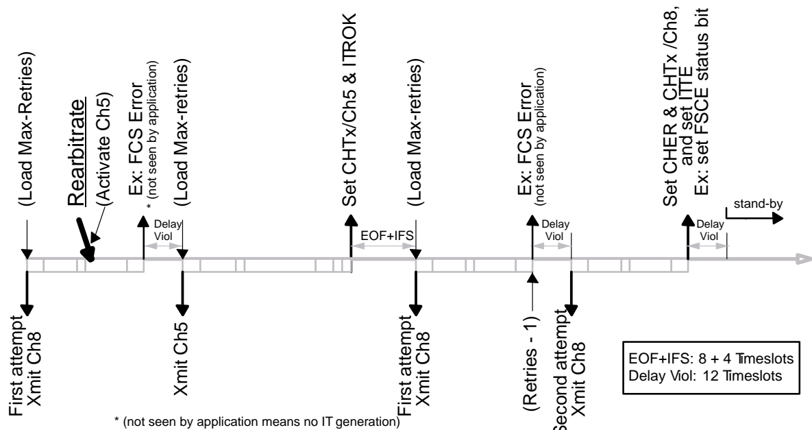
Figure 27. Rearbitrate Example
