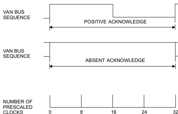
Figure 12. Acknowledge Sequences
