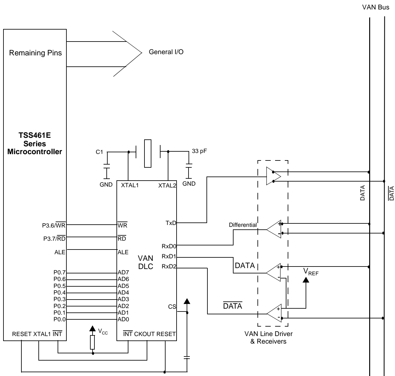
Figure 3. Typical Application
