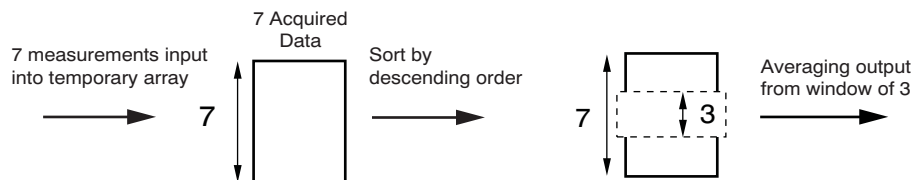
Figure 29. MAV Filter Operation (Patent Pending)
