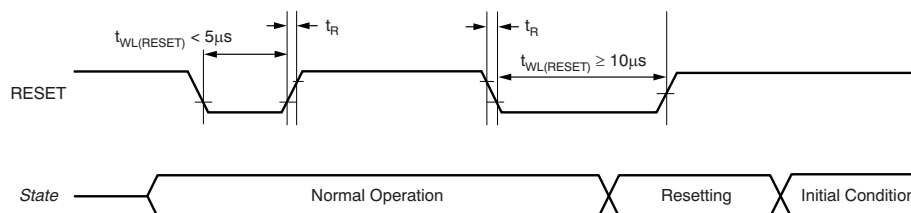
Figure 34. External Reset Timing
