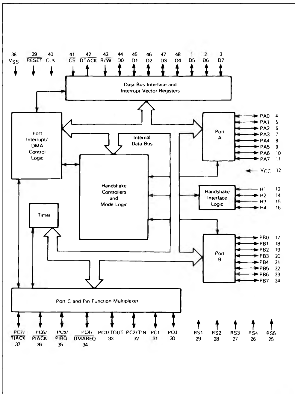
Figure 1.1 : Block Diagram.
