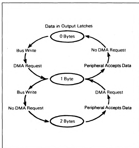
Figure 2.3 : DMAREQ Associated with Output Transfers.
