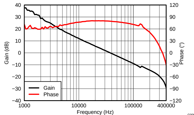
Figure 5. V OUT = 1.8 V, I OUT = 6 A, C OUT1 = 200 \mu F ceramic, f SW = 480 kHz
