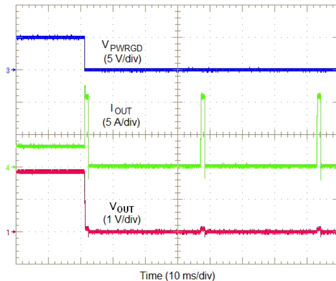
Figure 33. Overcurrent Limiting
