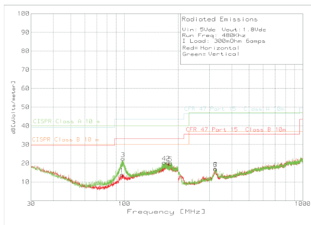
Figure 45. Radiated Emissions 5-V Input, 1.8-V Output, 6-A Load (EN55022 Class B)
