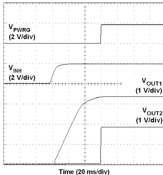
Figure 37. Sequencing Waveforms
