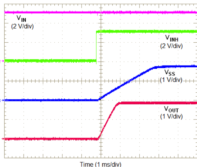
Figure 31. Inhibit Turn-On
