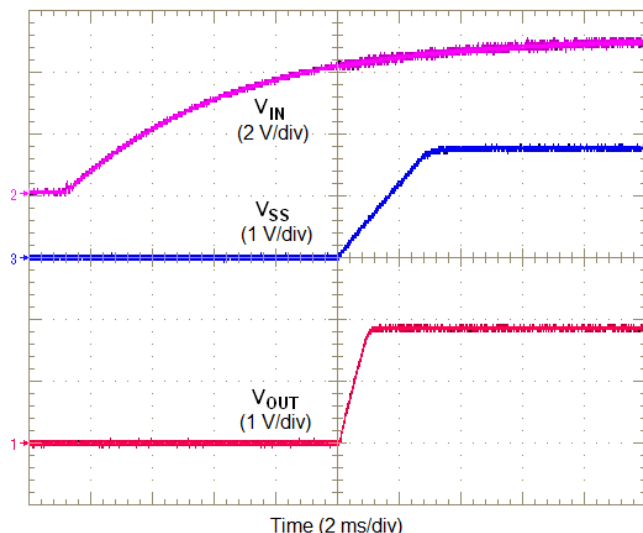
Figure 27. Start-Up Waveforms
