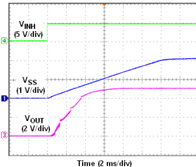
Figure 34. Inhibit Turn-On
