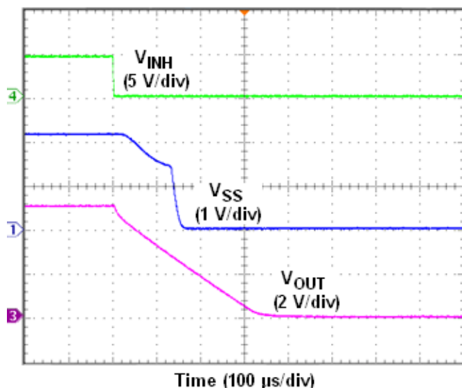
Figure 33. Inhibit Turn-Off
