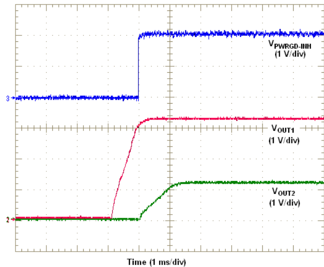
Figure 30. Sequencing Waveforms
