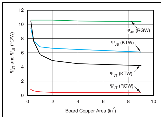
Figure 35. \Psi_{JT} and \Psi_{JB} vs Board Size
