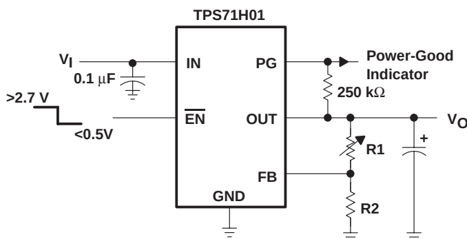
Figure 52. TPS71H01 Adjustable LDO Regulator Programming
