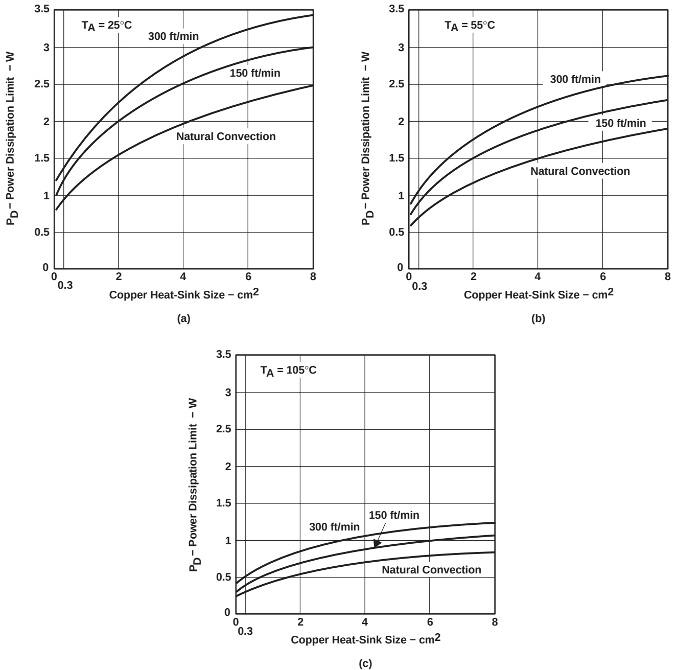
Figure 48. Power Ratings of the PWP Package at Ambient Temperatures of 25^\circ\text{C} , 55^\circ\text{C} , and 105^\circ\text{C}
