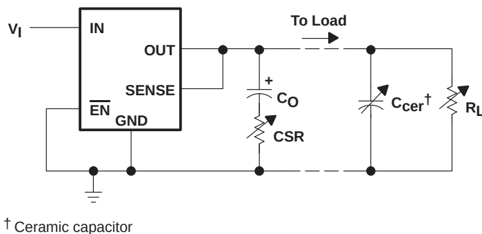
Figure 42. Test Circuit for Typical Regions of Stability (see Figures 34 through 41)
