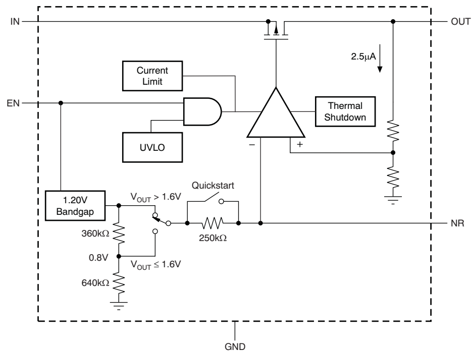
Figure 1. Fixed Voltage Versions
