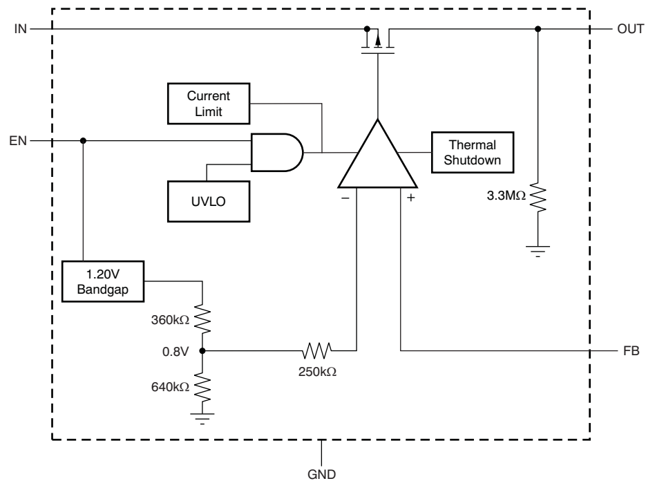
Figure 2. Adjustable Voltage Version
