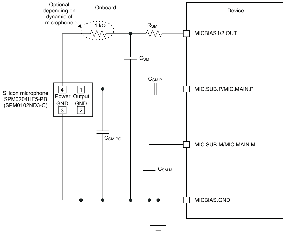
Figure 5-26. Silicon Microphone
