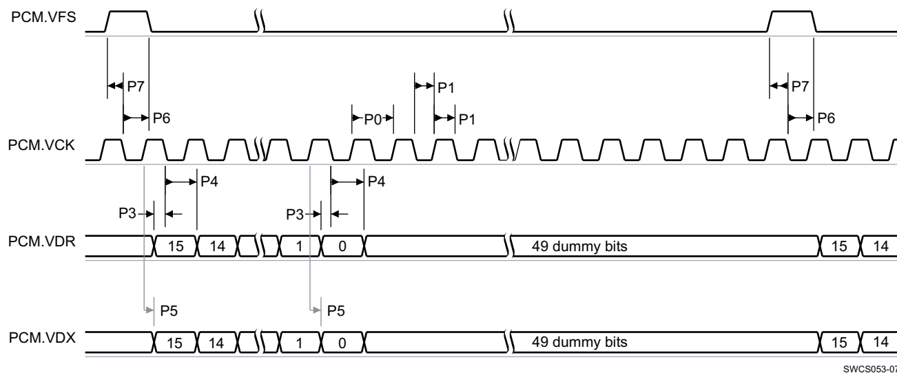
Figure 7-9. Voice PCM Interface—Slave Mode (Mode 1)
