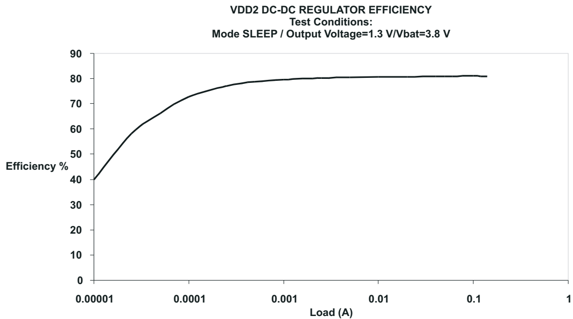
Figure 6-6. VDD2 DC-DC Regulator Efficiency in Sleep Mode
