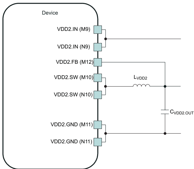
Figure 6-7. VDD2 DC-DC Application Schematic
