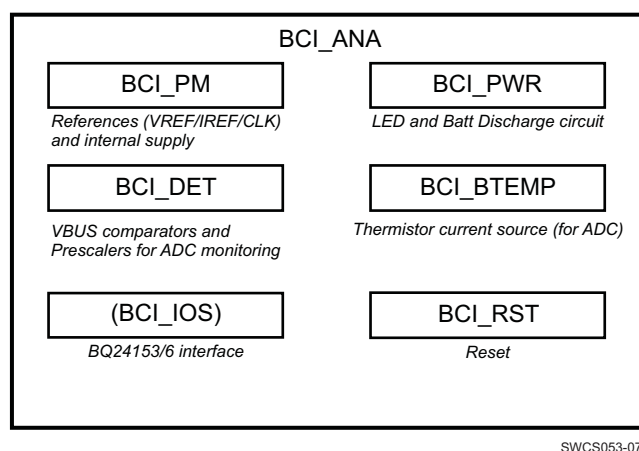
Figure 8-1. Battery Charger Block Diagram
