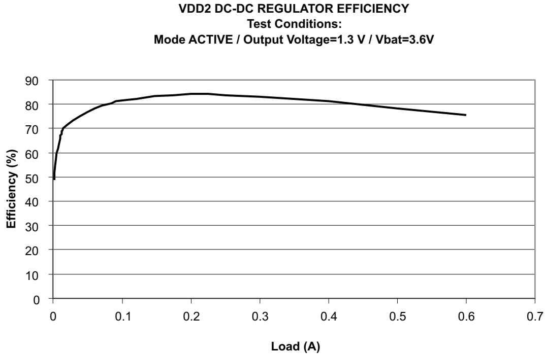
Figure 6-5. VDD2 DC-DC Regulator Efficiency in Active Mode
