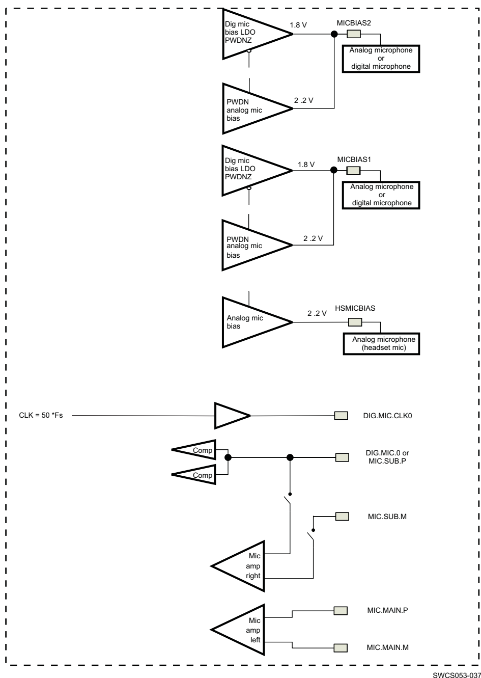
Figure 5-21. Analog and Digital Microphone Muxing
