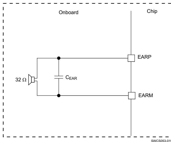
Figure 5-3. Earphone Speaker
