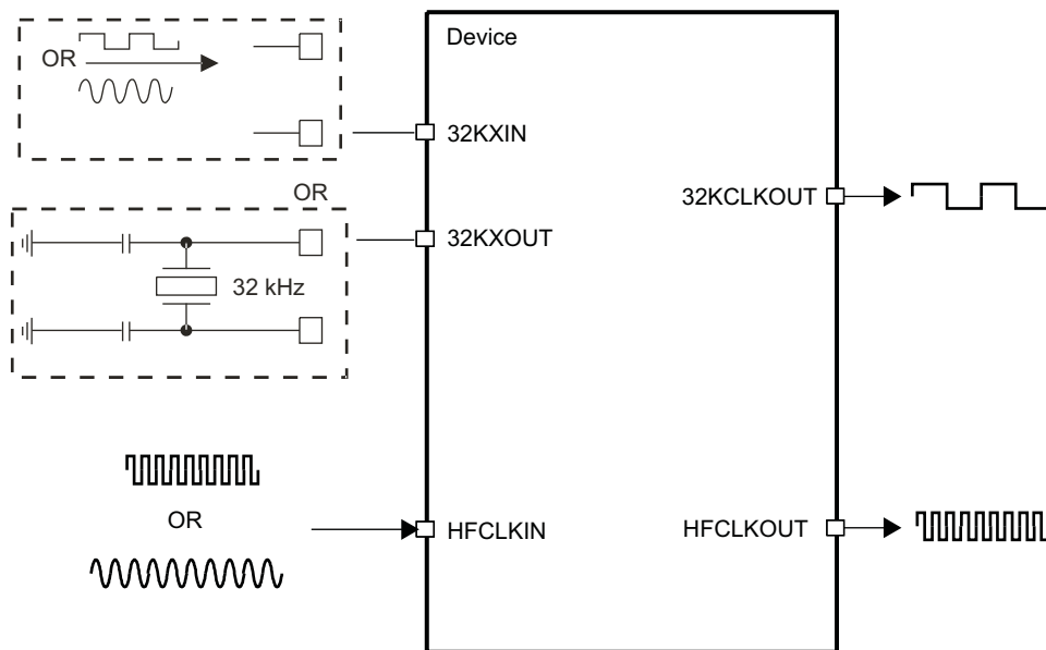
Figure 4-1. Clock Overview
