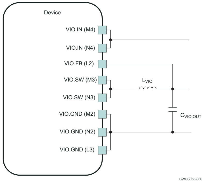
Figure 6-10. VIO DC-DC Application Schematic
