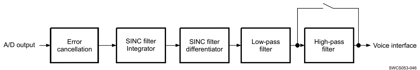
Figure 5-31. Digital Audio Filter Uplink Path Characteristics
