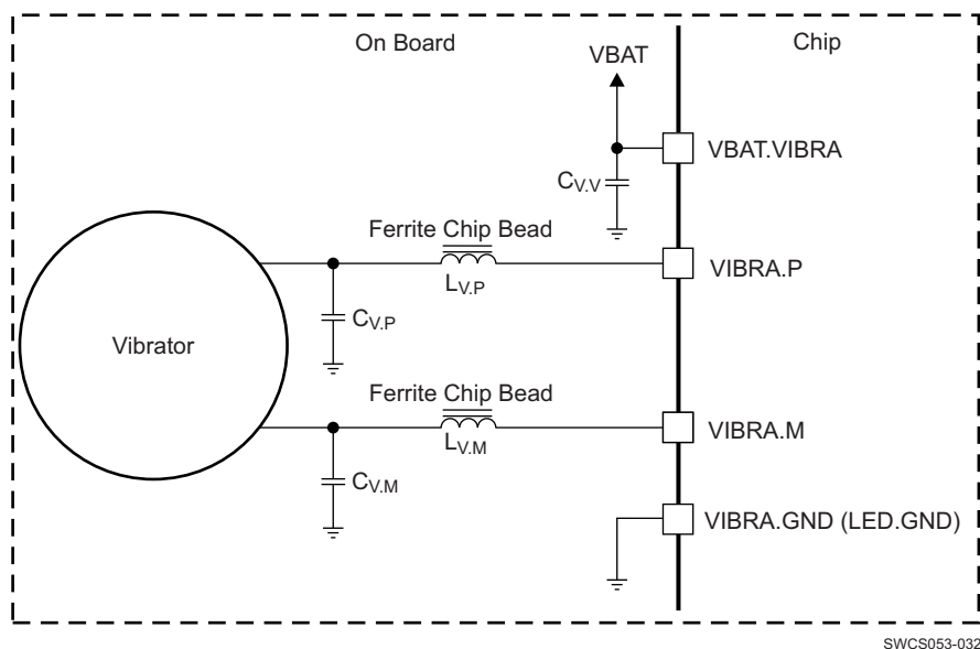
Figure 5-16. Vibra H-Bridge
