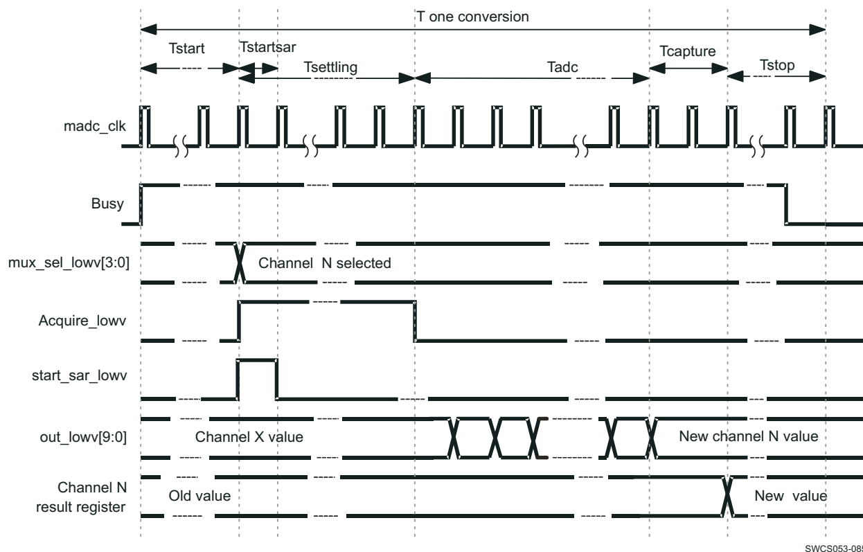
Figure 9-1. One Conversion Sequence General Timing Diagram
