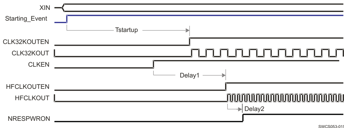
Figure 4-14. 32KCLKOUT and HFCLKOUT Clock Stabilization Time
