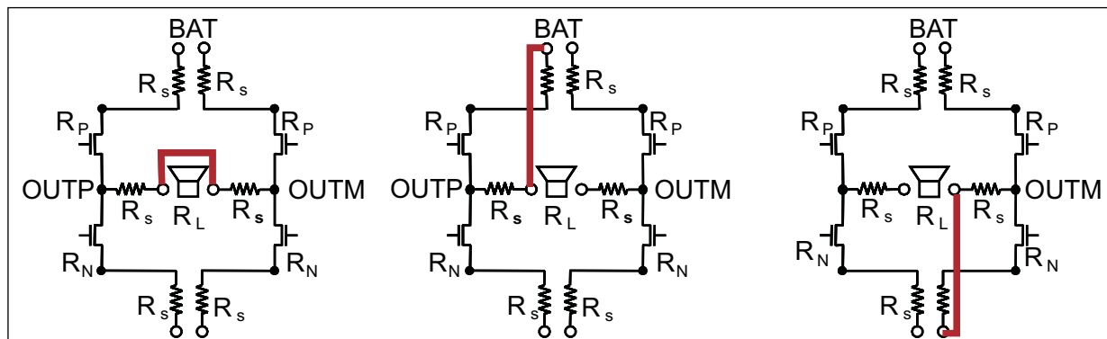
Figure 5-5. Class-D: Short-Circuits
