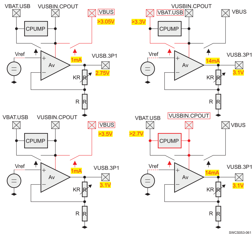
Figure 6-11. VUSB3V1 LDO Supply Selection for the Different Modes of Operation
