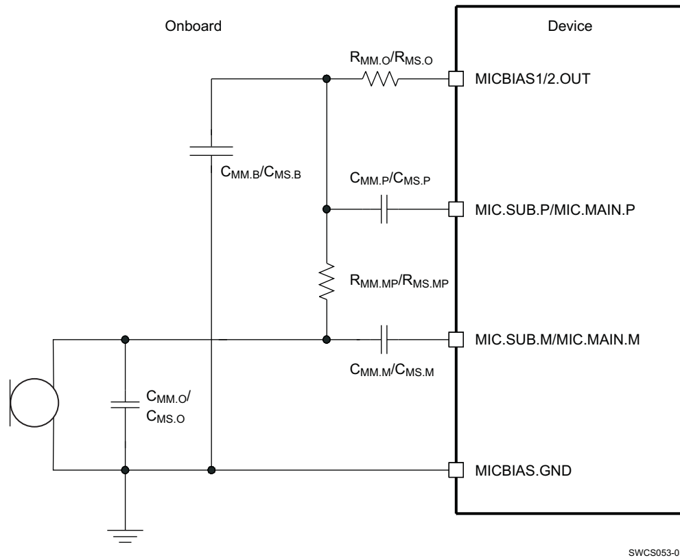
Figure 5-22. Analog Microphone Pseudodifferential
