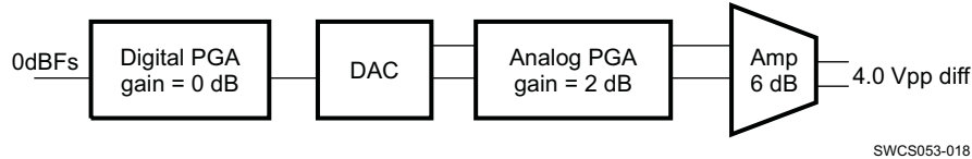
Figure 5-2. Earphone Amplifier
