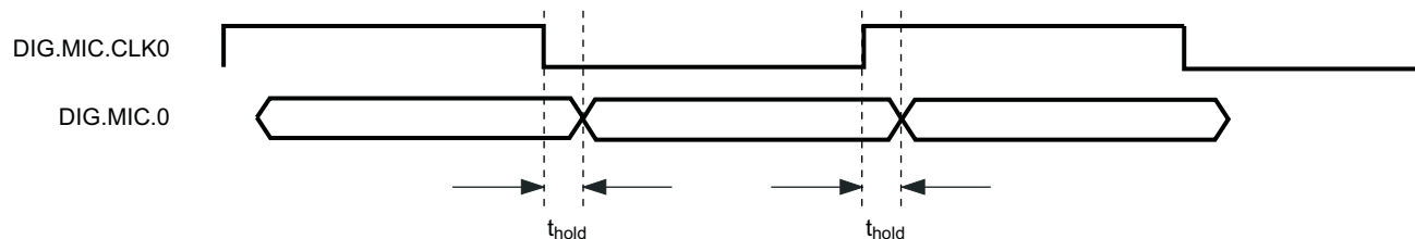
Figure 5-25. Digital Microphone Timing Diagram
