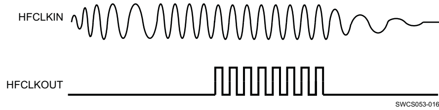
Figure 4-15. HFCLKOUT Behavior
