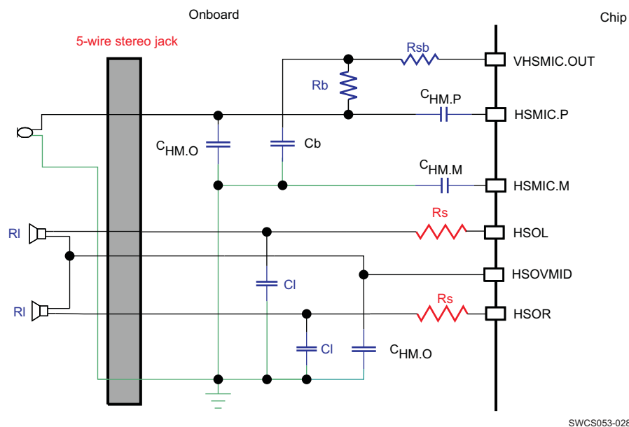
Figure 5-12. Headset 5-Wire Stereo Jack
