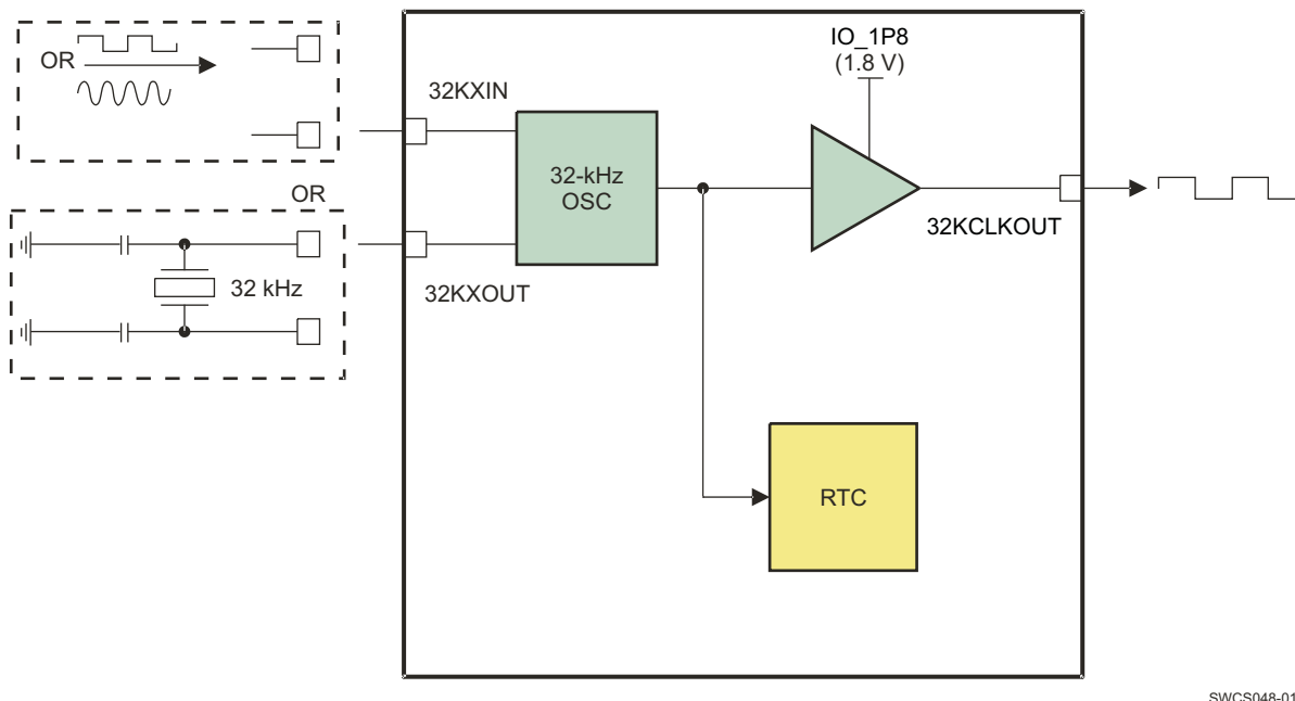
Figure 12. 32.768-kHz Clock Output Block Diagram
