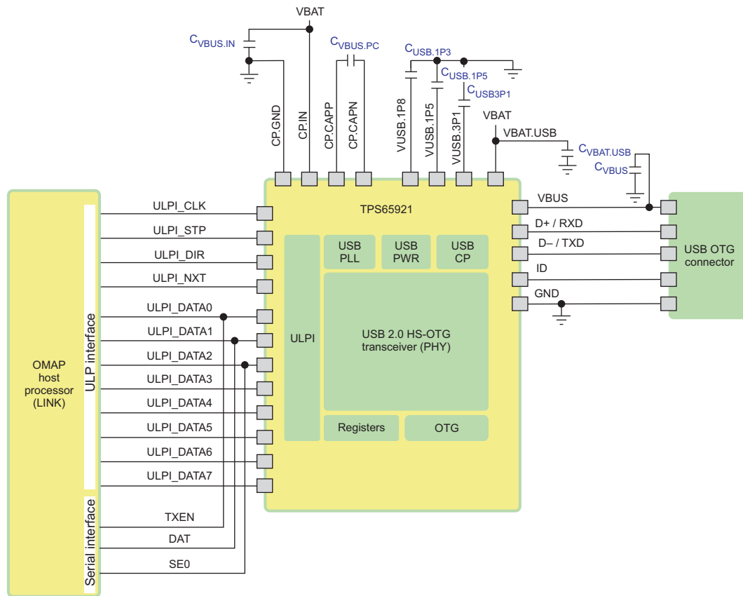
Figure 23. USB System Application Schematic
