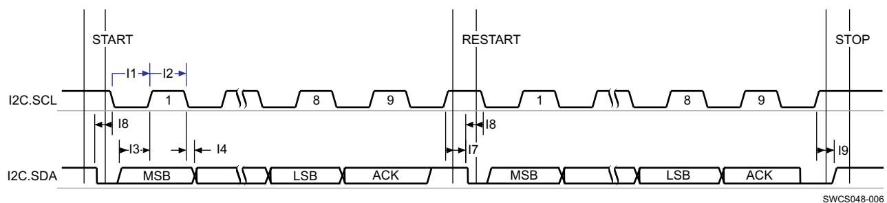
Figure 6. I 2 C Interface—Transmit and Receive in Slave Mode
