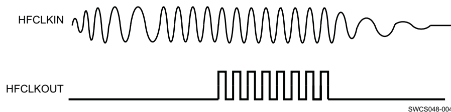
Figure 4. HFCLKOUT Behavior
