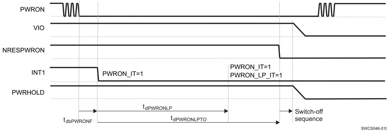
Figure 6. PWRON Long-Press Turn-Off
