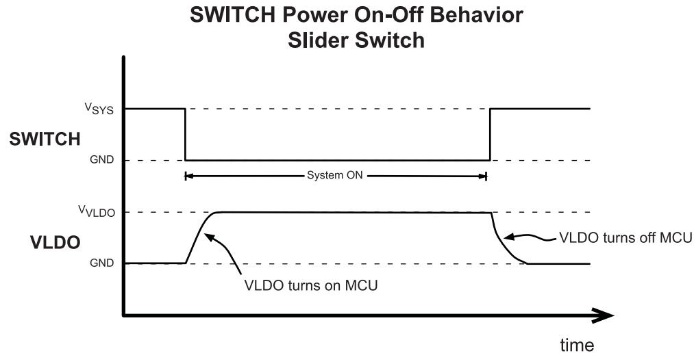
Figure 2-15. SWITCH, Slider Power On-Off Behavior
