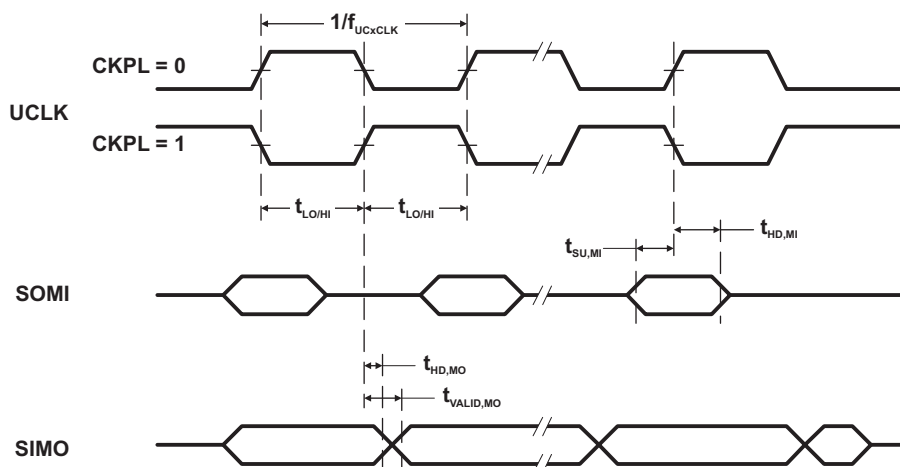
Figure 3-17. SPI Master Mode, CKPH = 1
