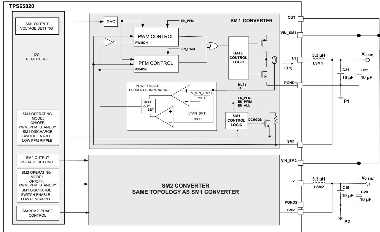
Figure 42. SM1/SM2 Converter
