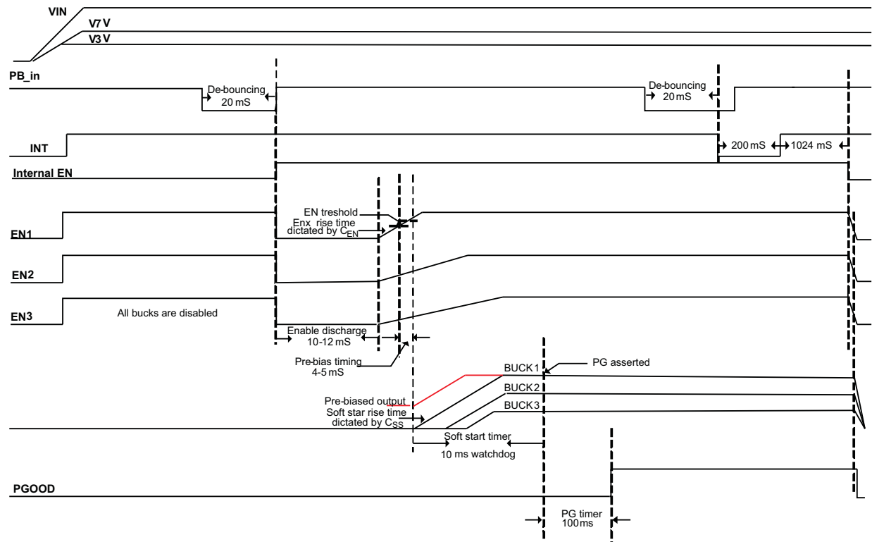
Figure 41. Delayed Start-Up
