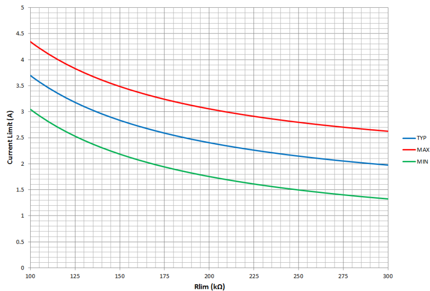
Figure 35. Buck 3
