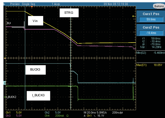
Figure 44. Dump Operation
