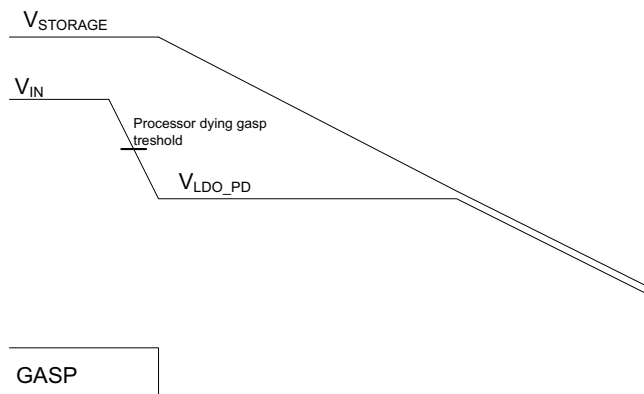
Figure 2. Pump and Dump Mode
