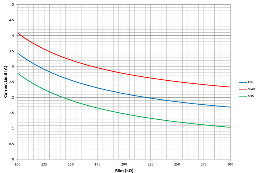
Figure 34. Buck 2
