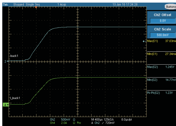
Figure 6. Start-Up V_{OUT} = 1.2\text{ V} , 3.5\text{ A}
