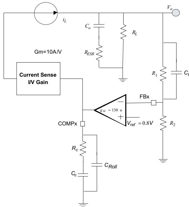
Figure 32. Loop Compensation
