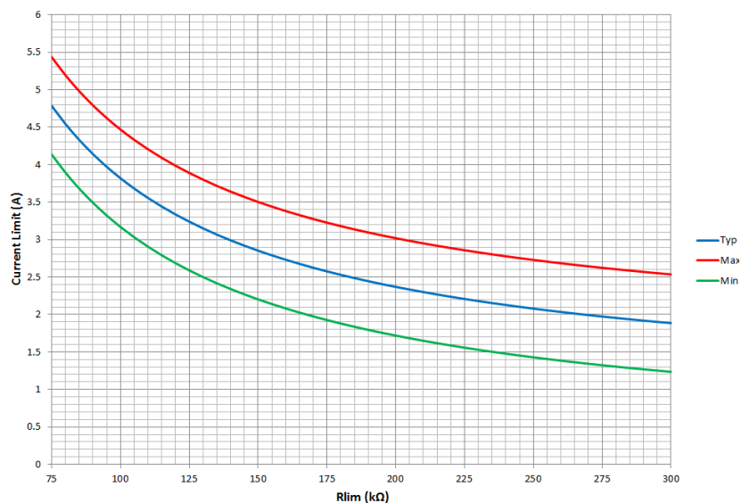
Figure 33. Buck 1
