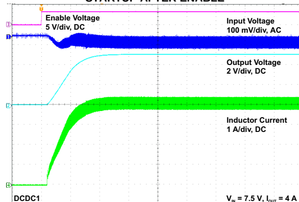
Time 200 \mu\text{s/div} Figure 2-44.
