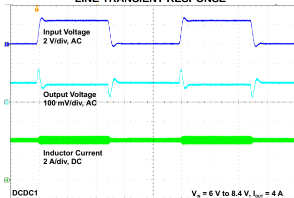
Time 200 \mu\text{s/div} Figure 2-41.
