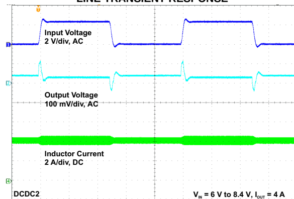
Time 200 \mu\text{s/div} Figure 2-42.
