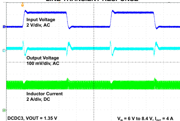
Time 200 \mu\text{s/div} Figure 2-43.
