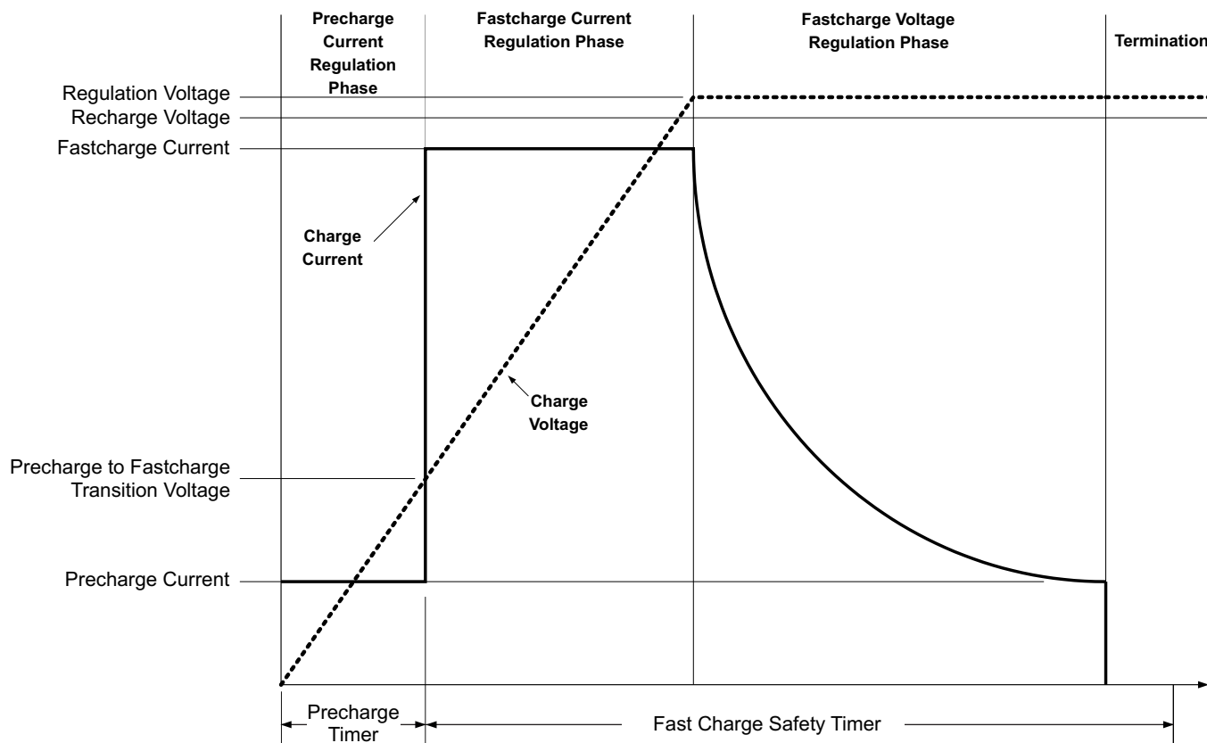
Figure 3-8. Charging Cycle
