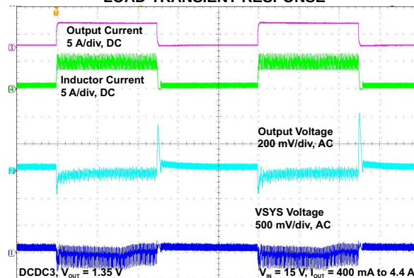
Time 200 \mu\text{s/div} Figure 2-40.
