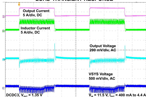
Time 200 \mu\text{s/div} Figure 2-39.
