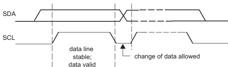
Figure 3-2. Bit Transfer on the I²C-bus
