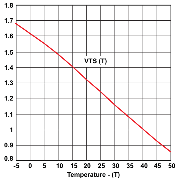
Figure 48. Resulting TS Voltage
