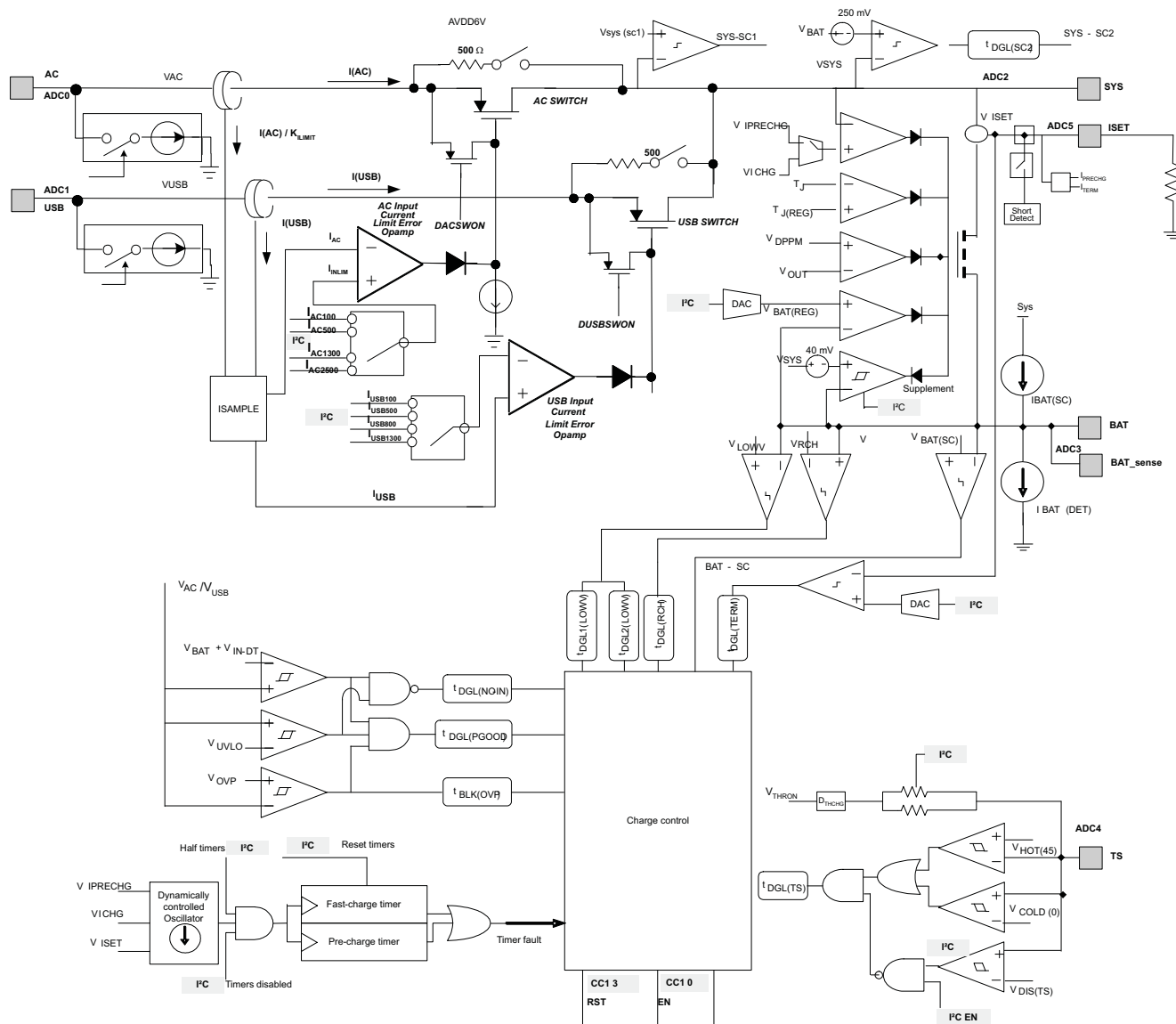
Figure 25. Charger Block Diagram
