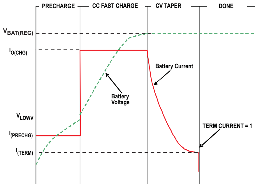
Figure 27. Battery Charge
